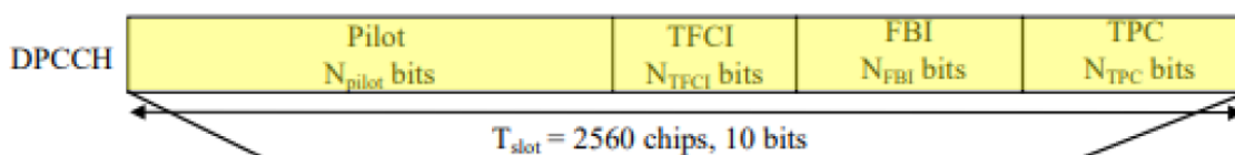
Ex.2014, Detail of FIG. 1 (annotated)
