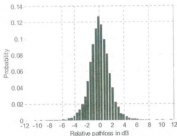
Figure 4. Distribution of relative pathloss in dB in Case 1
