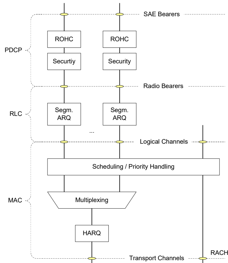
Figure 8.2: Layer 2 Structure for UL in UE
