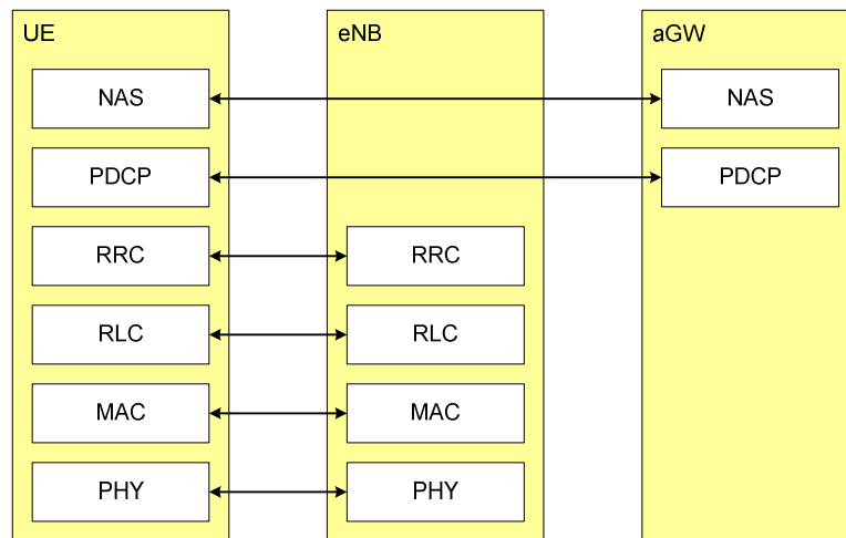
Figure 6.3: C-plane protocol stack
