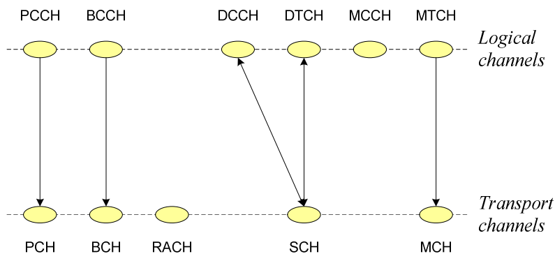
Figure 8.3: Mapping between logical channels and transport channels
