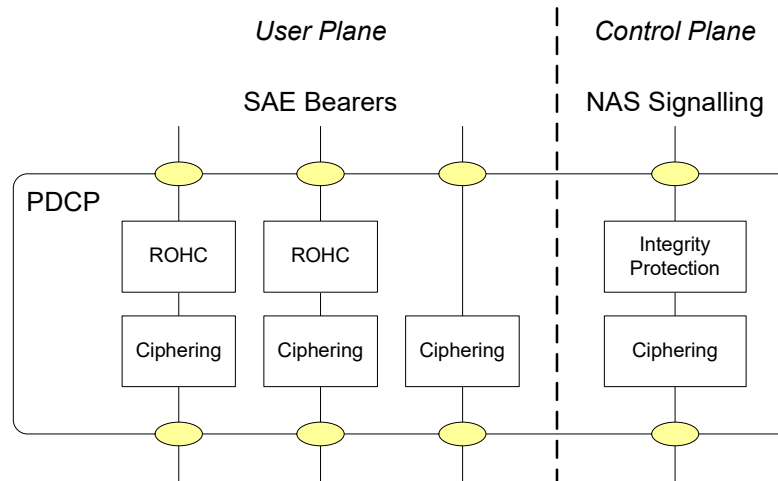
Figure 8.4: Model of PDCP sublayer
