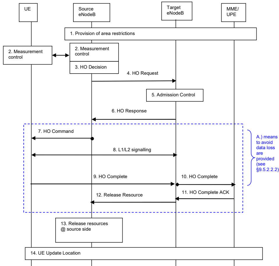
Figure 9.2: Information flow for Intra-LTE-Access Mobility Support
