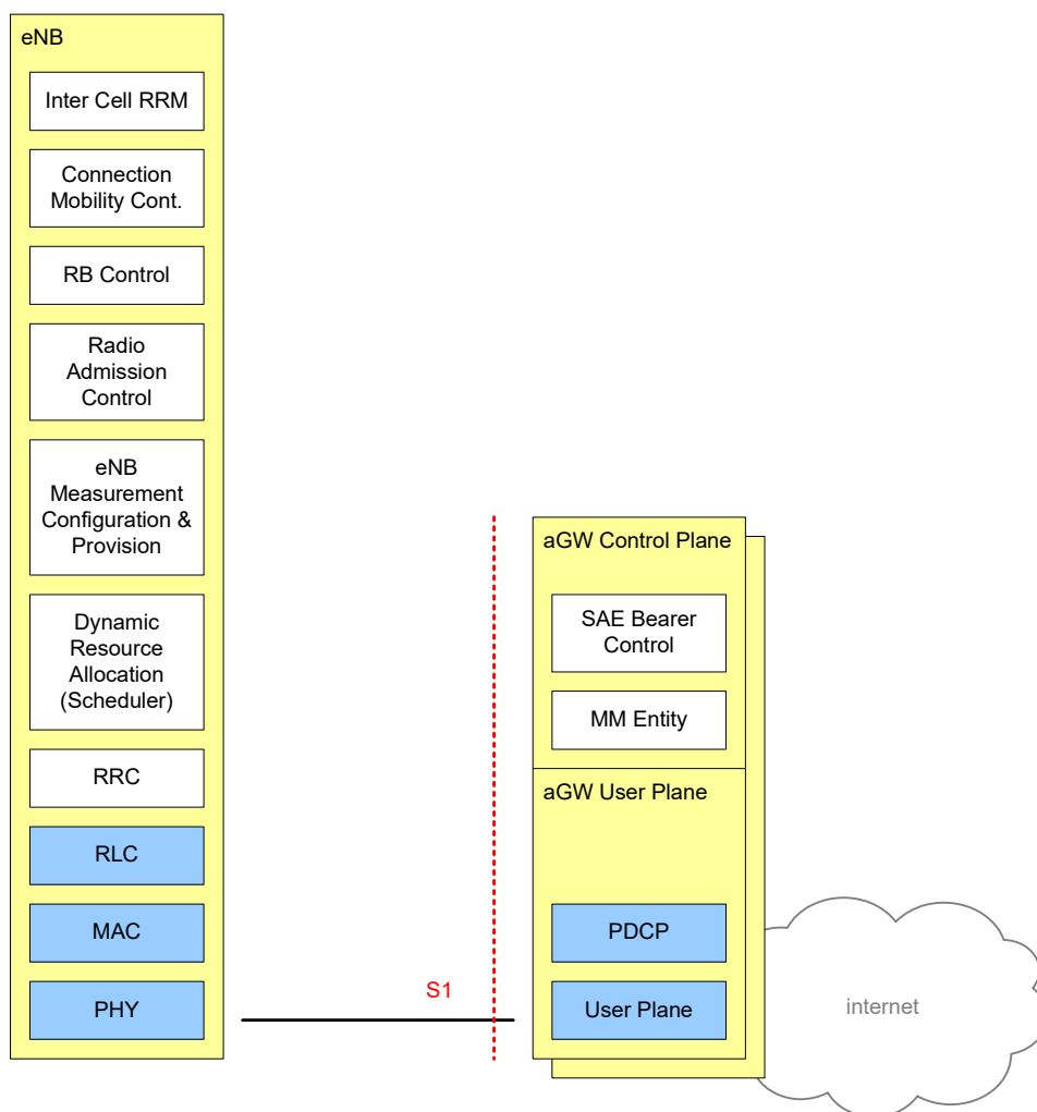
Figure 6.1: E-UTRAN Architecture
