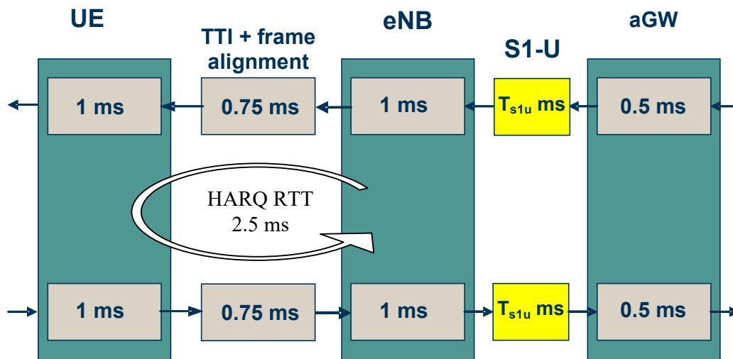
Figure 13.2: U-plane latency components in LTE
