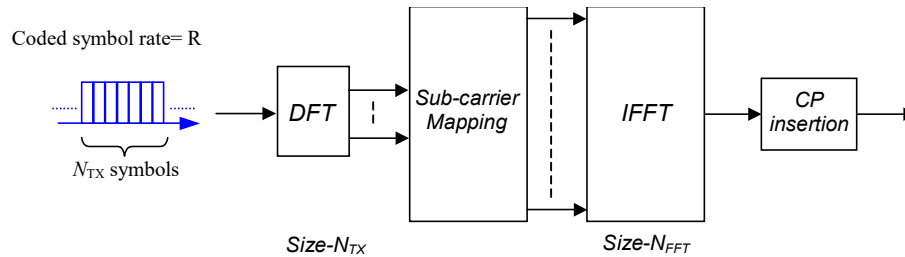
Figure 7.2: Transmitter structure for SC-FDMA.
