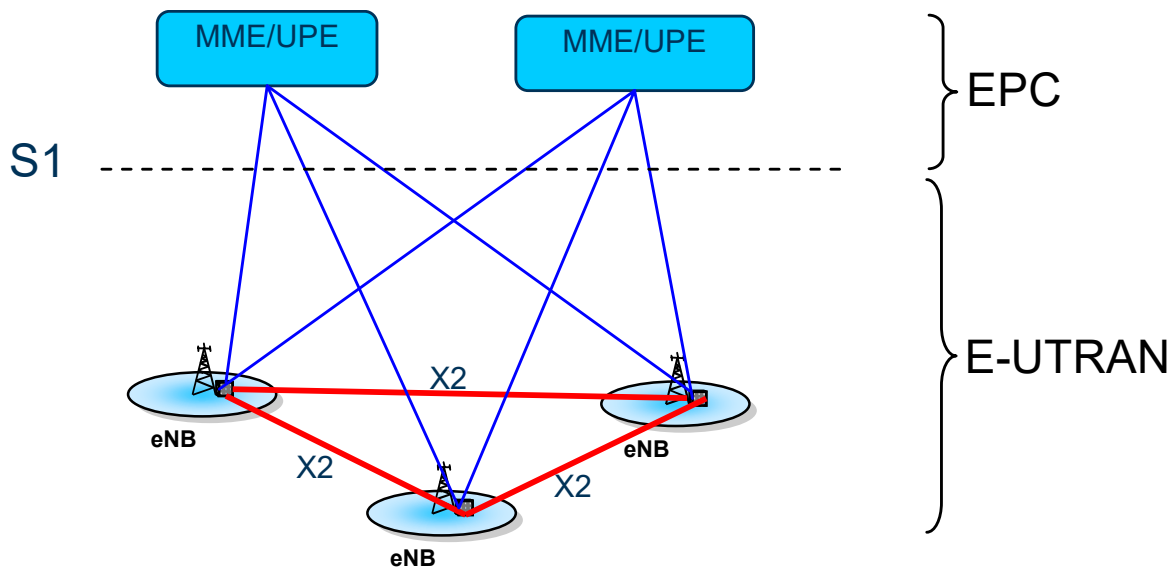
Figure 9.1: E-UTRAN architecture
