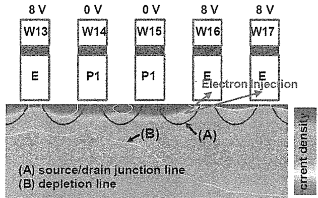
FIGURE 6.65 Device simulation is performed on the BV_{dss} measurement condition at PP1 pattern. Current density shows the punch-through of WL15 off-cell at V_{bl} = 4\text{ V} . DIBL (drain-induced barrier lowering) generates punch-through between source and drain in unselected cell. Electrons generated by punch-through are injected at nearby cells (disturb happens). Lower V_t cell shows larger DIBL.
