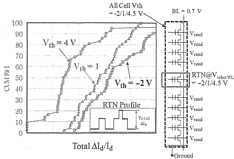
FIGURE 8.38 The cumulative curves of current fluctuation ( = total \Delta I_d / I_d ) at the same current ( I_d = 100 nA) according to cell states of 40 cells. Inset shows the schematic picture of RTN profile.
