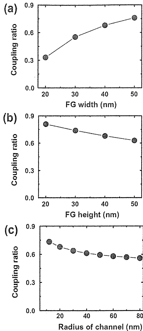
FIGURE 7.59 Coupling ratio of the DC-SF cell in case of T_{ox} = 8 nm and T_{IPD} = 12 nm. (a) Coupling ratio of the DC-SF cell as a function of FG width ( a_3 - a_2 ) (FG height: 40 nm and radius of channel poly: 20 nm). (b) Coupling ratio of the DC-SF cell as a function of FG height ( h ) (FG width, 40 nm; radius of channel poly, 20 nm). (c) Coupling ratio of DC-SF cell as a function of radius of channel poly ( a_1 ) (FG height, 40 nm; FG width, 40 nm).
