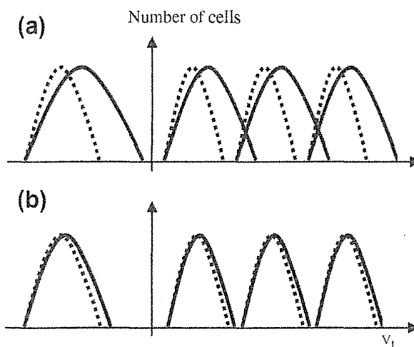
FIGURE 7.65 Cell threshold voltage ( V_t ) setting comparison between: (a) conventional planar FG cell with large FG-FG coupling interference and (b) DC-SF cell with small FG-FG coupling interference. The DC-SF cell has a wider V_t setting margin due to negligible FG-FG coupling.
