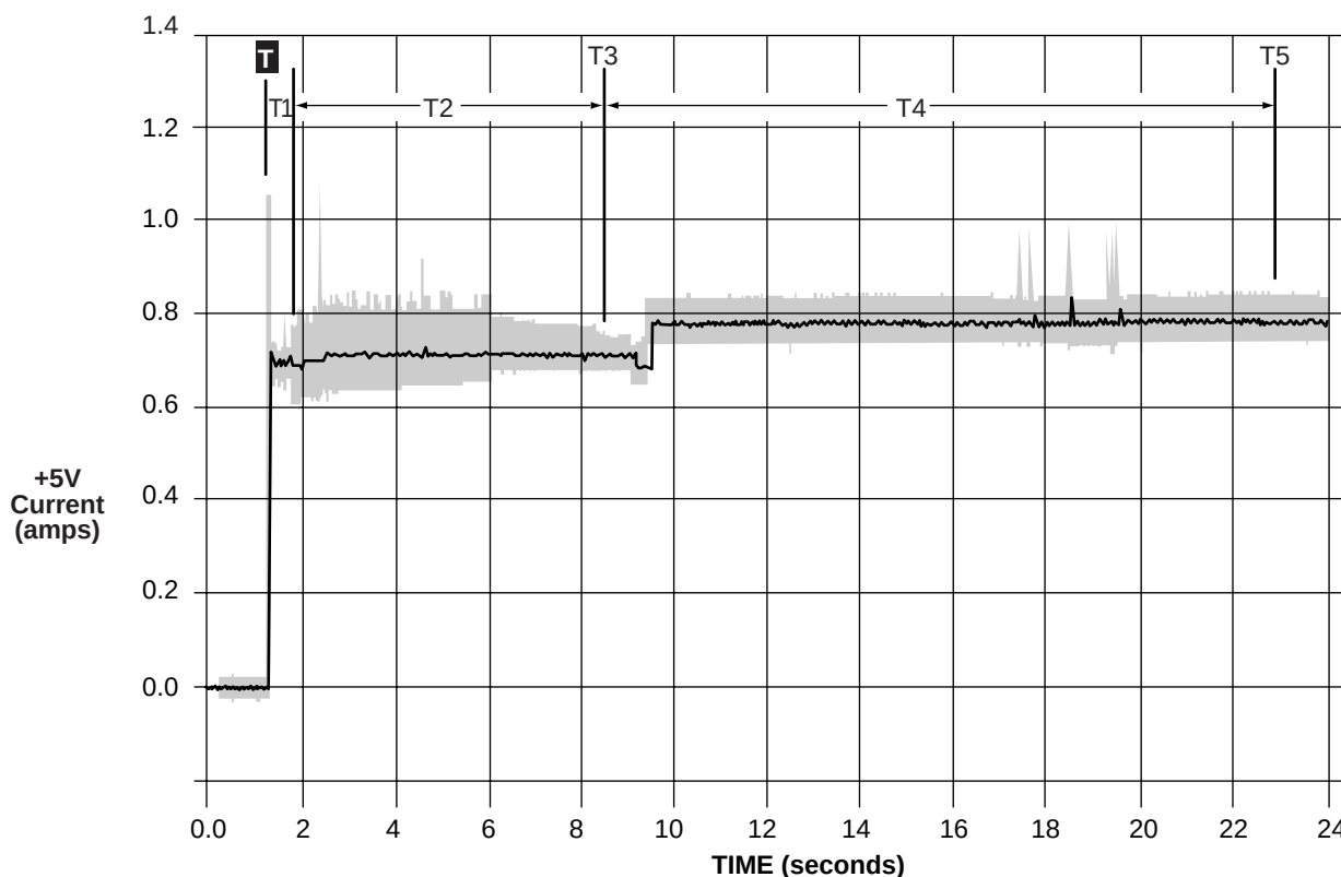
Figure 3b. Typical Barracuda 9LP family drive +5 V current profile
