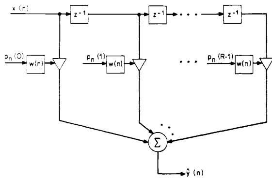
Fig. 4. Block diagram of the effects (in time) of making modifications to the short-time spectrum for the OLA method.
