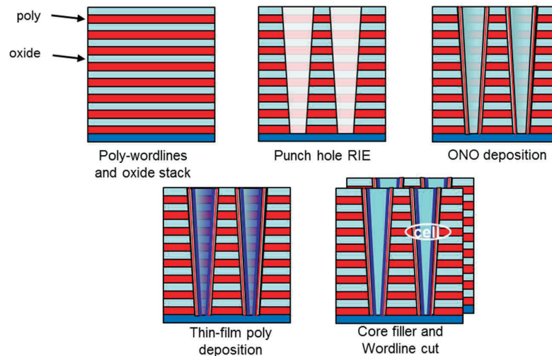
Figure 2. Punch-and-plug process steps (gate first).
