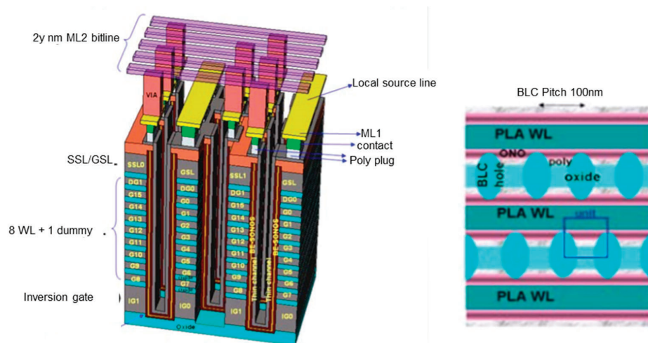
Figure 12. Single-gate vertical channel (SGVC) [33].
