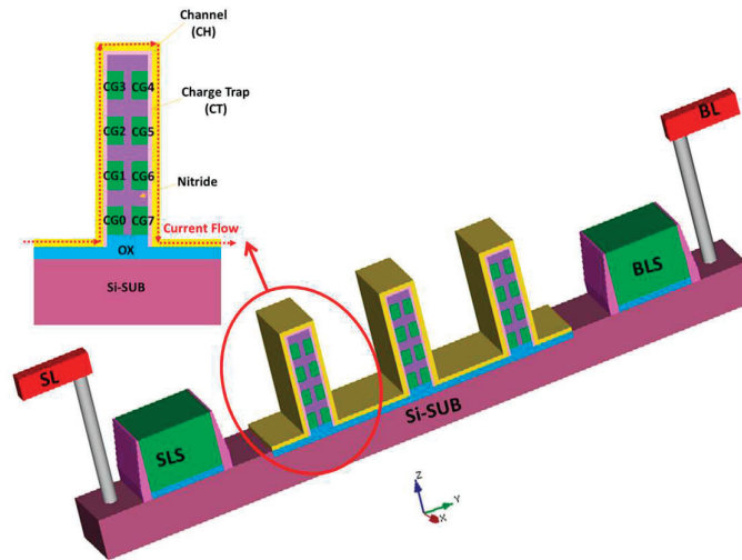
Figure 10. VSAT architecture.
