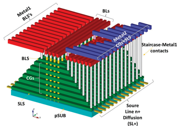
Figure 7. V-NAND structure [copyright 2016 by Springer] [4].
