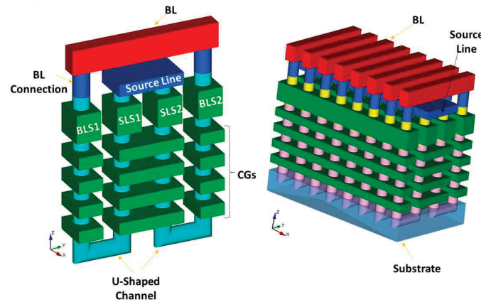
Figure 6. PBiCS structure.
