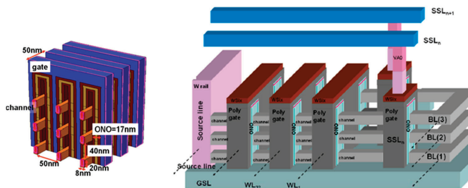
Figure 11. 3D vertical-gate (VG) NAND [27].
