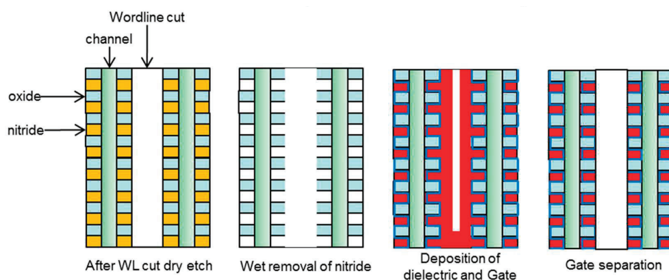
Figure 8. TCAT/V-NAND process.
