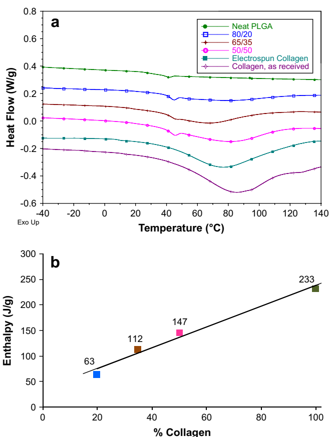
Fig. 5. DSC thermogram of neat as well as blends of PLGA and Collagen (a) and trend in enthalpy of denaturation of collagen (b).
