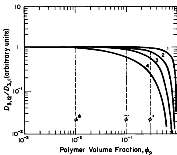
Fig. 8. The effect of the equilibrium polymer volume fraction \phi_2 on the normalized solute diffusivity in hydrogels when r = 0.1\xi (1), 0.2\xi (2), 0.3\xi (3), and 0.4\xi (4). Experimental data are available between \phi_2 = 5 \times 10^{-2} and \phi_2 = 7 \times 10^{-1} .
