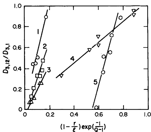
Fig. 6. Dependence of the normalized diffusion coefficient D_{3,12}/D_{3,1} on the term (1 - r/\xi)\exp[-1/(Q - 1)] . Data presented are for (1) salicylic acid (correlation coefficient \rho = 0.975 ) through PHEMA, 29 (2) progesterone ( \rho = 0.982 ) through p(\text{HEMA-co-MEMA}) hydrogels with EGMA, 28 (3) progesterone ( \rho = 0.953 ) through p(\text{HEMA-co-MEMA}) hydrogels with TEGDMA, 28 (4) theophylline ( \rho = 0.991 ) through PVA, 25 and (5) bovine serum albumin ( \rho = 0.953 ) through PVA. 26
