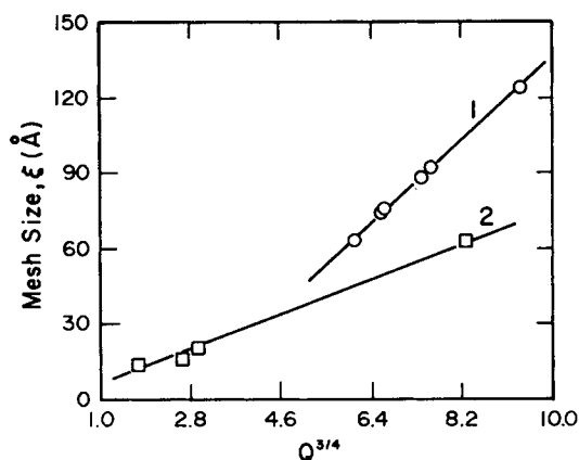
Fig. 5. Mesh sizes vs. equilibrium volume degree swelling Q , plotted as Q^{3/4} , in semidilute gels of PHEMA (1) and PVA (2). Correlation coefficients are 0.998 and 0.996, respectively. Data from Refs. 25 and 26.
