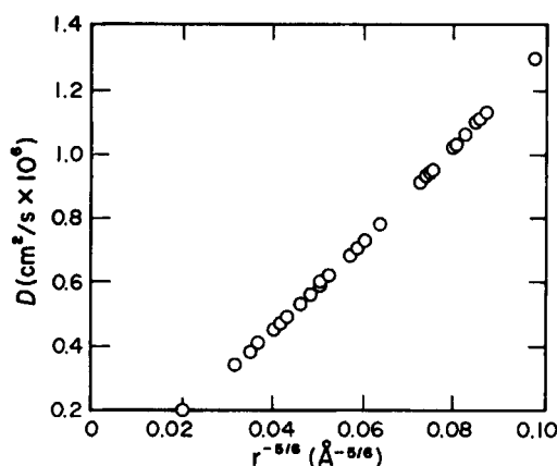
Fig. 1. Overall dependence of the solute diffusion coefficient, D_{3,12} ( \text{cm}^2/\text{s} ), on the solute size, r ( \text{\AA} ), in deionized water at 20^\circ\text{C} .
