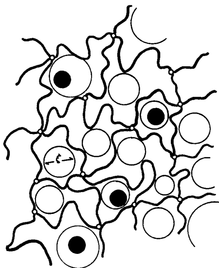
Fig. 3. Crosslinked structure of a polymer gel, showing effective chains of the structure defined by crosslinks. The effective area for diffusion for the solute is characterized by an average mesh size \xi . The smaller solutes, illustrated as dark circles, must pass between the macromolecules.
