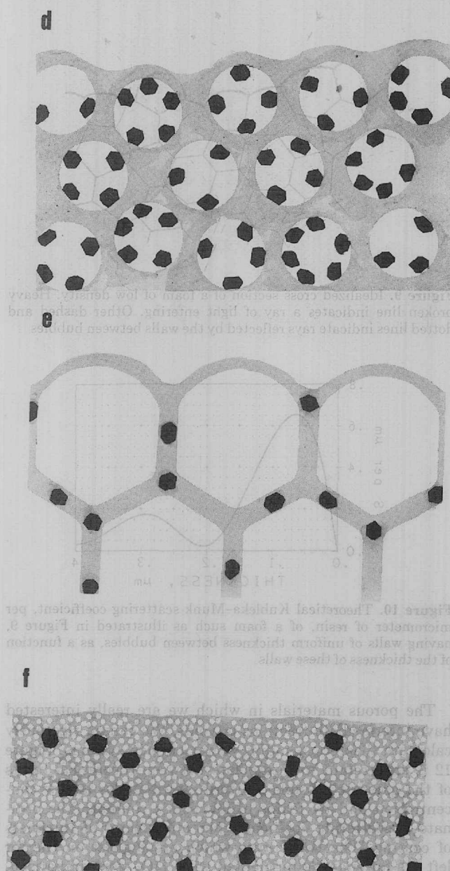
Figure 14. Idealized cross sections illustrating possible types of distributions of \text{TiO}_2 particles in foams. Black represents \text{TiO}_2 , gray represents resin, and white represents air. See text for discussion of differences.
