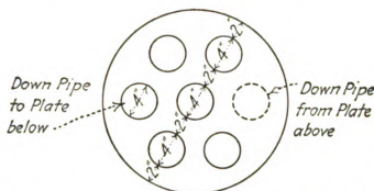
FIG. 27.—Arrangement of caps on plate.
