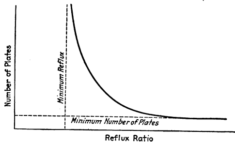
FIG. 21.—Curve showing relation between reflux ratio and number of plates.
