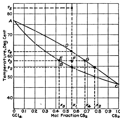
Fig. 5.—Boiling point curve for \text{CCl}_4 — \text{CS}_2 mixtures.
