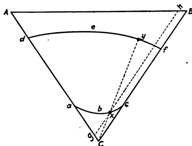
FIG. 11.—Constant temperature diagram. Three component space model.
