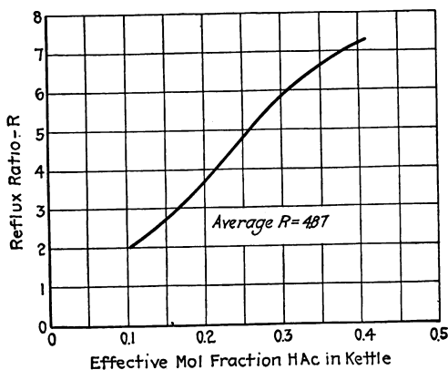
FIG. 26.—Plot of reflux ratio versus concentration in kettle.
