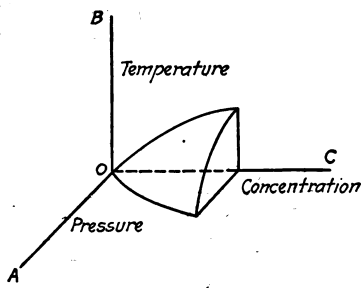
FIG. 3.—Space model—two component system.
