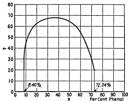
FIG. 4.—Solubility curve of phenol-water mixtures.
