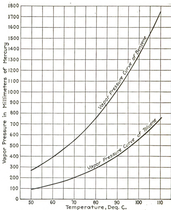
FIG. 12.—Vapor pressure curves of benzene and toluene.
