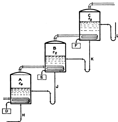
FIG. 7.—Diagram of multiple distillation.
