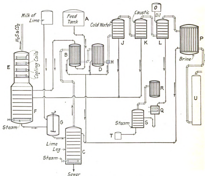
FIG. 32.—Continuous ammonia still.
