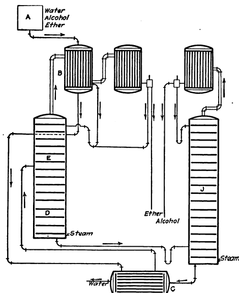
FIG. 30.—Type B—continuous still for three components.
