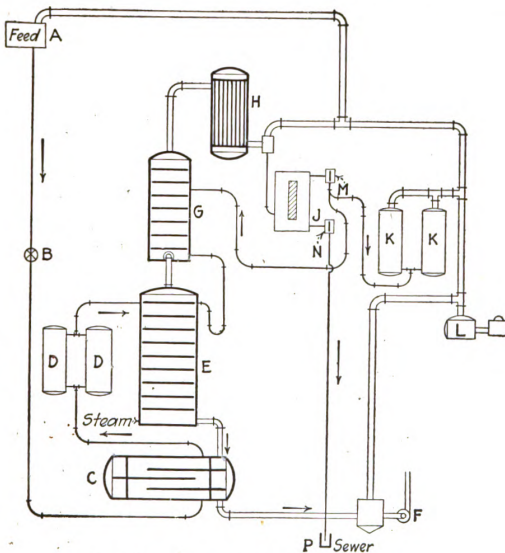
FIG. 35.—Vacuum wash oil still.
