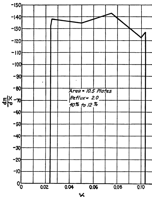
FIG. 24.—Plot of \frac{dn}{dx} versus x .
