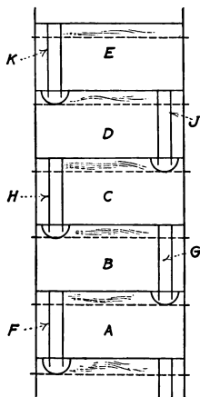
FIG. 8.—Diagram of fractionating column.
