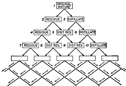
FIG. 6.—Fractionation diagram.
