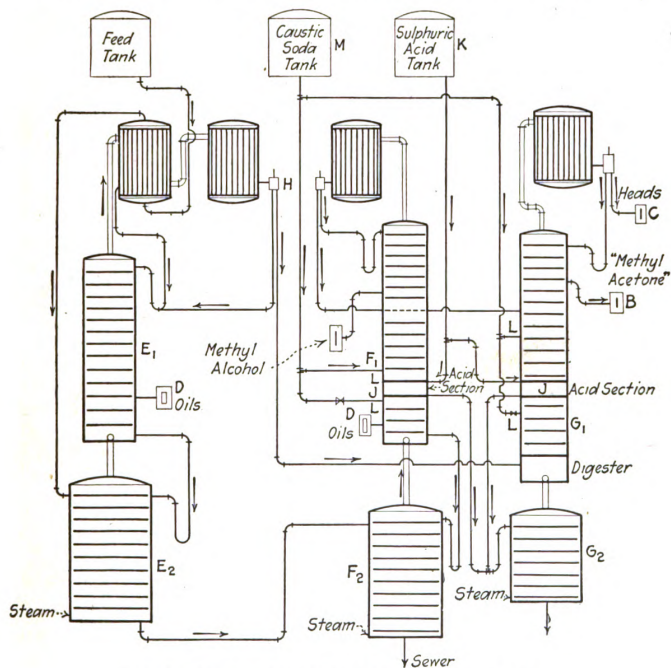
FIG. 36.—Continuous methyl alcohol-acetone still.
