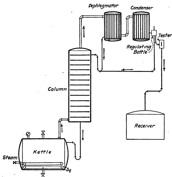
FIG. 38.—Modern intermittent still.
