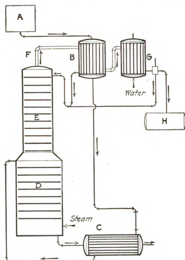
FIG. 28.—Diagram of a simple continuous still.
