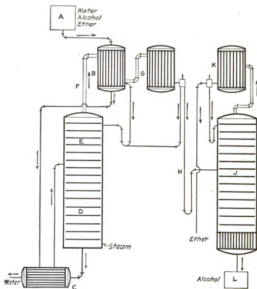
Fig. 29.—Type A—continuous still for three components.
