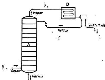
FIG. 17.—Diagram of fractionating column.
