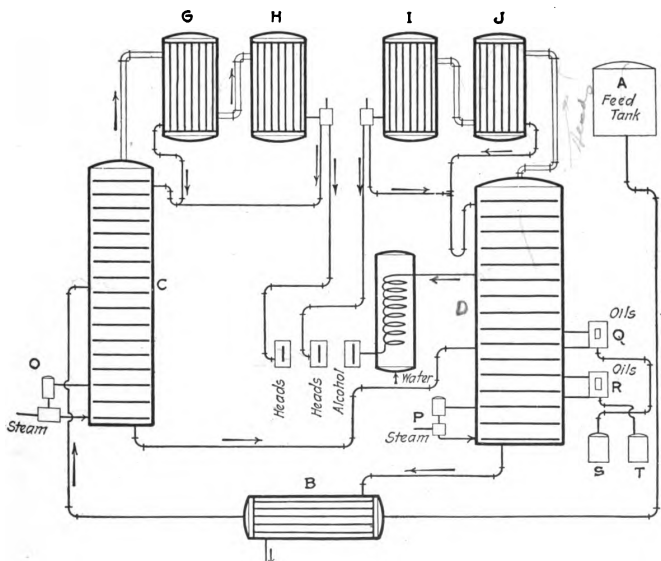
FIG. 39.—Continuous ethyl alcohol still.
