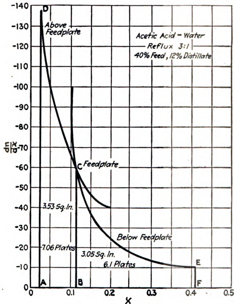
FIG. 20.—Plot of \frac{dn}{dx} and \frac{dm}{dx} versus x (reduced scale).
