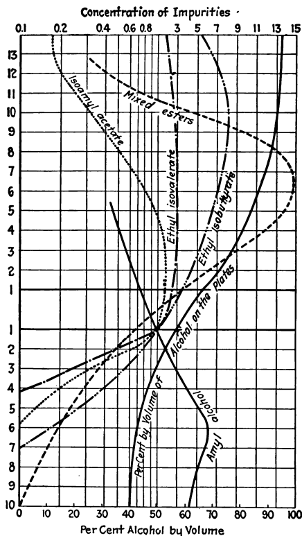
FIG. 40.—Diagram illustrating action of purifying column.
