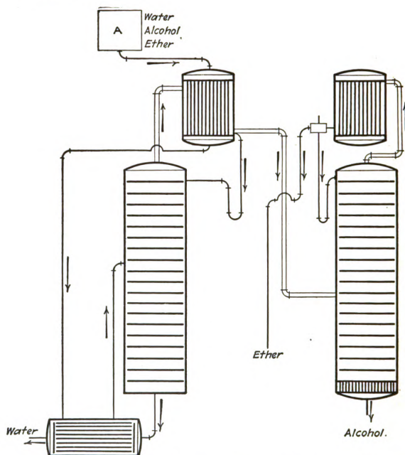
FIG. 31.—Type C—continuous still for three components.
