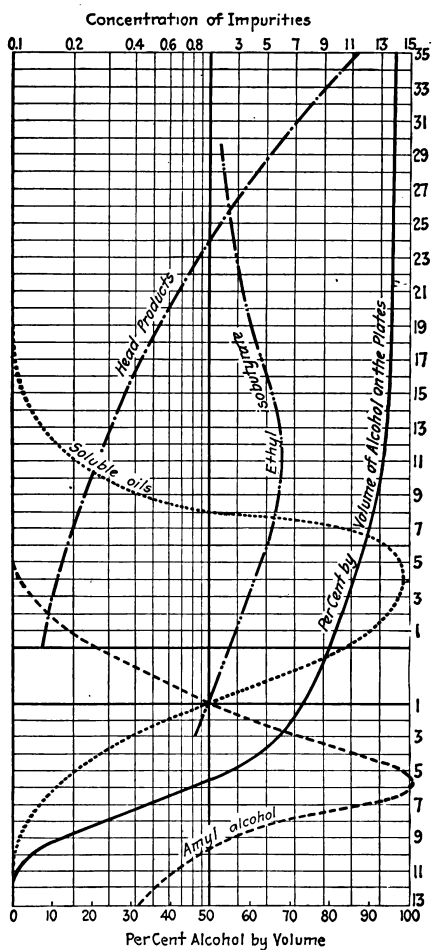
FIG. 41.—Diagram illustrating action of rectifying column.
