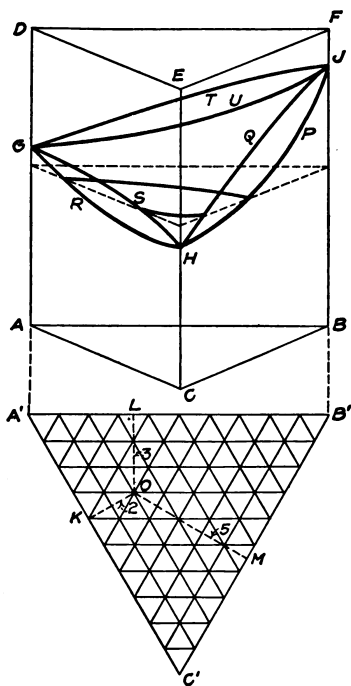
FIG. 10.—Diagram of three component system.
