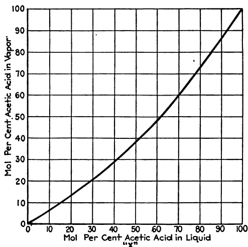
FIG. 18.—Vapor composition curve for acetic acid-water mixtures.
