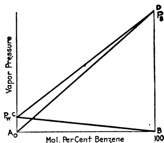
FIG. 33.—Vapor pressure relations. Benzene—wash oil mixtures.
