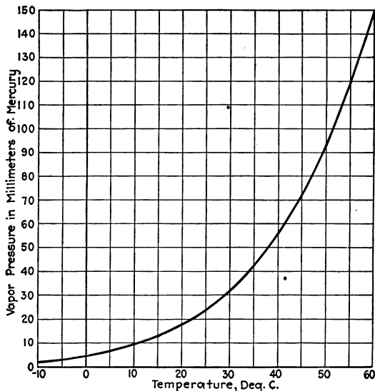
FIG. 1.—Vapor pressure curve of water.
