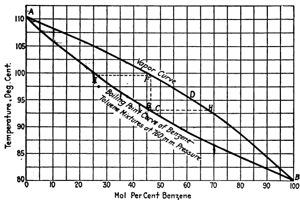
FIG. 14.—Boiling point curve for benzene-toluene mixtures.
