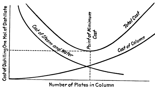
FIG. 22.—Optimum number of plates in fractionating column.
