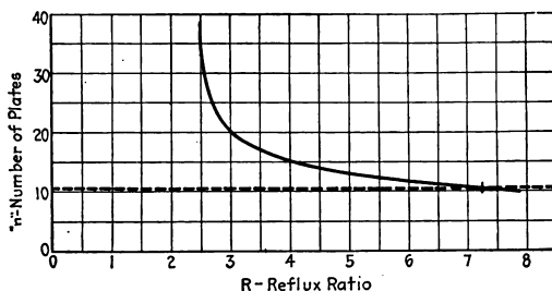
FIG. 25.—Plot of reflux ratio versus number of plates.
