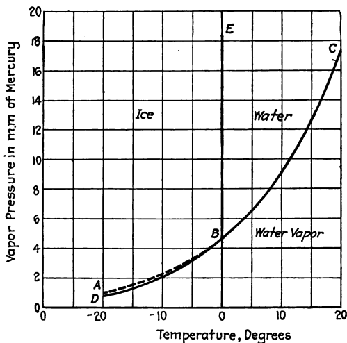
FIG. 2.—Vapor pressure diagram. System—ice, water, water vapor.
