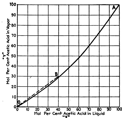
FIG. 15.—Liquid-vapor composition curve for acetic acid-water mixtures.
