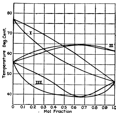
FIG. 9.—Types of binary mixtures.
