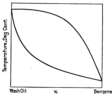
FIG. 34.—Boiling point curve. Benzene—wash oil mixtures.
