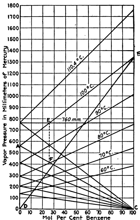
Fig. 13.—Partial pressure curves of benzene—toluene mixtures.
