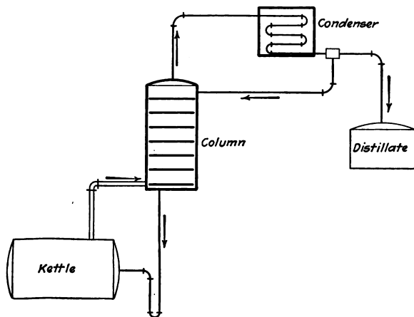
FIG. 23.—Diagram of an intermittent still.
