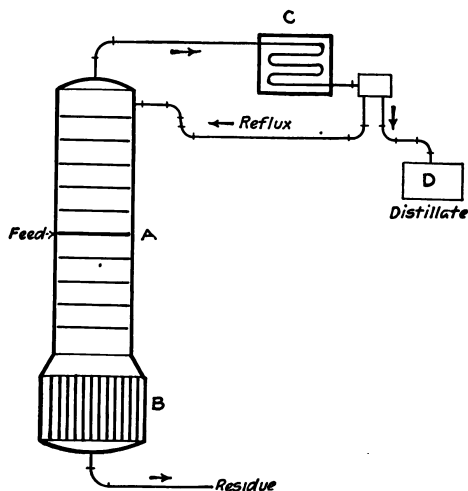
FIG. 19.—Diagram of continuous still
