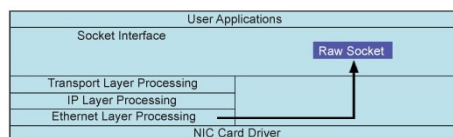
Figure 1: Graphical demonstration of a raw socket
