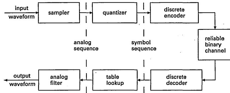
Figure 4.1. Encoding and decoding a waveform source.
