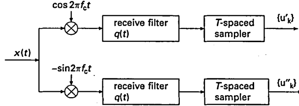
Figure 6.8. DSB-QC demodulation.
