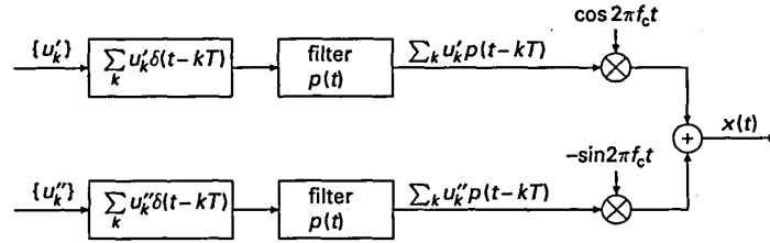
Figure 6.7. DSB-QC modulation.
