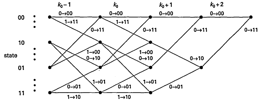
Figure 8.10. Trellis termination.
