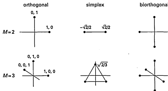
Figure 8.6. Orthogonal, simplex, and biorthogonal signal constellations.
