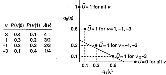
Figure 8.12. Error curve for a discrete observation space. There are only five points making up the “curve,” one corresponding to each of the five distinct threshold rules. For example, the threshold rule \tilde{U} = 1 only for v = -3 yields (q_1(\eta), q_0(\eta)) = (0.6, 0.1) for all \eta in the range 1/4 to 2/3 . A straight line of slope -\eta through that point is also shown for \eta = 1/2 . Lemma 8.10.1 asserts that this line lies on or beneath each point of the error curve and each point (q_1(A), q_0(A)) for any other test. Note that as \eta increases or decreases, this line will rotate around the point (0.6, 0.1) until \eta becomes larger than 2/3 or smaller than 1/4 ; it then starts to rotate around the next point in the error curve.
