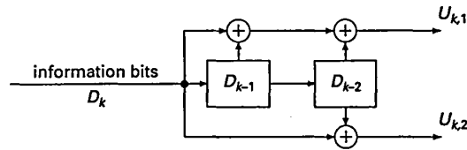
Figure 8.8. Example of a convolutional code.
