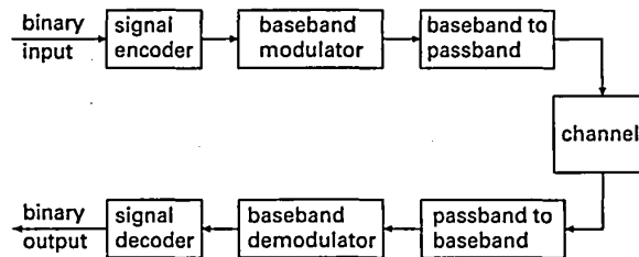
Figure 6.5. QAM modulator and demodulator.
