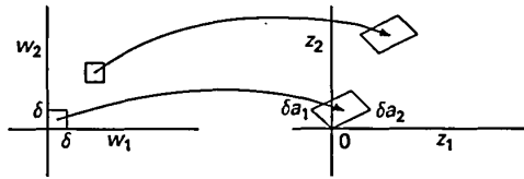
Figure 7.1. Example illustrating how Z = AW maps cubes into parallelepipeds. Let Z_1 = -W_1 + 2W_2 and Z_2 = W_1 + W_2 . The figure shows the set of sample pairs z_1, z_2 corresponding to 0 \leq w_1 \leq \delta and 0 \leq w_2 \leq \delta . It also shows a translation of the same cube mapping into a translation of the same parallelepiped.
