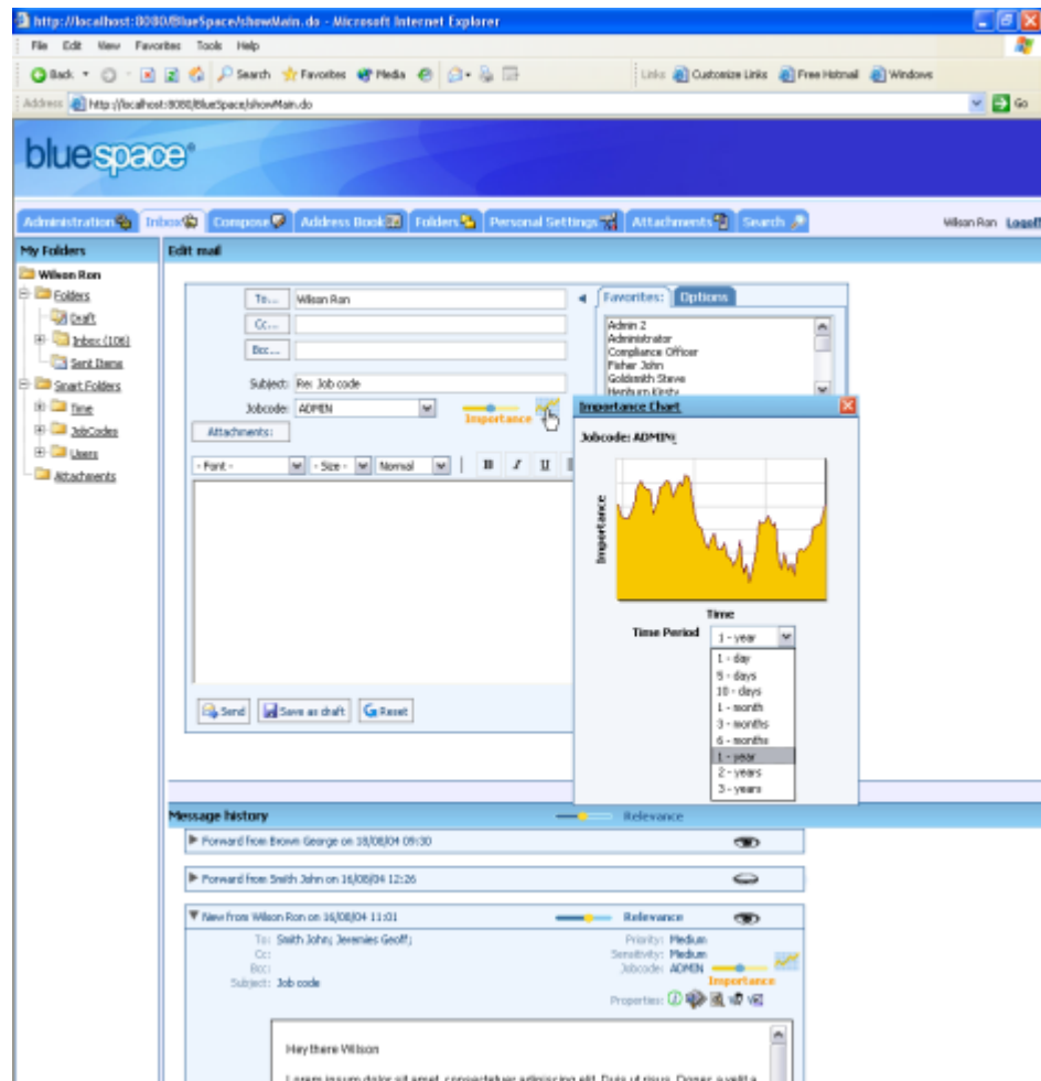
Figure 11 – Importance evolution
