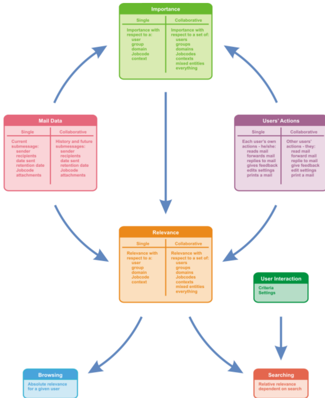
Figure 6 – Relevance overview
