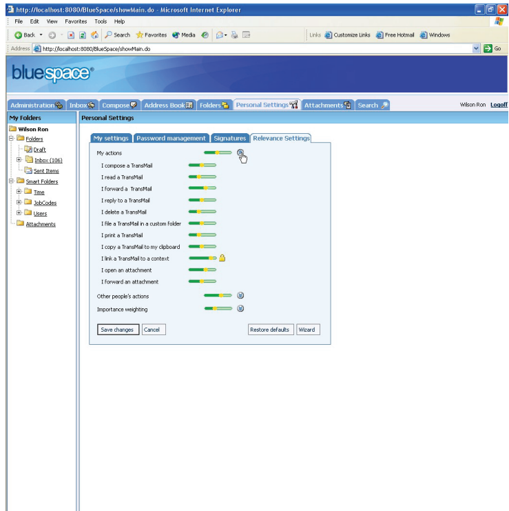
Figure 14 – Tuning the algorithm
