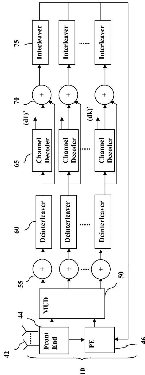
Figure 1 (Prior Art)
