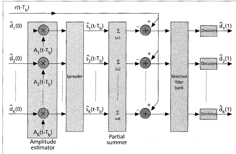
■ Figure 6. One stage of a PIC detector (hard decision) for K users. The initial stage (conventional detector) is not shown; it introduces one bit delay, which is why the received signal and the amplitudes are delayed by T_b . The spreader is defined in Fig. 3 and the matched filter bank is defined in Fig. 1.
