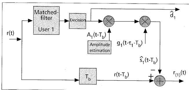
■ Figure 5. SIC detection – first stage (hard decision).
