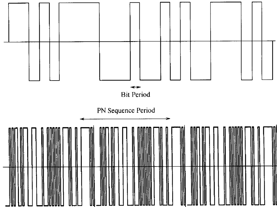
FIGURE 2.9. Direct-sequence spread spectrum system with N_0 = 63 and N = 7 .
