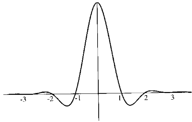
FIGURE 1.12. Raised cosine pulse with \alpha = 0.5 .
