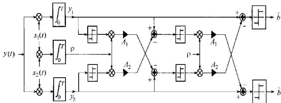
FIGURE 7.16. Three-stage detector for two synchronous users.
