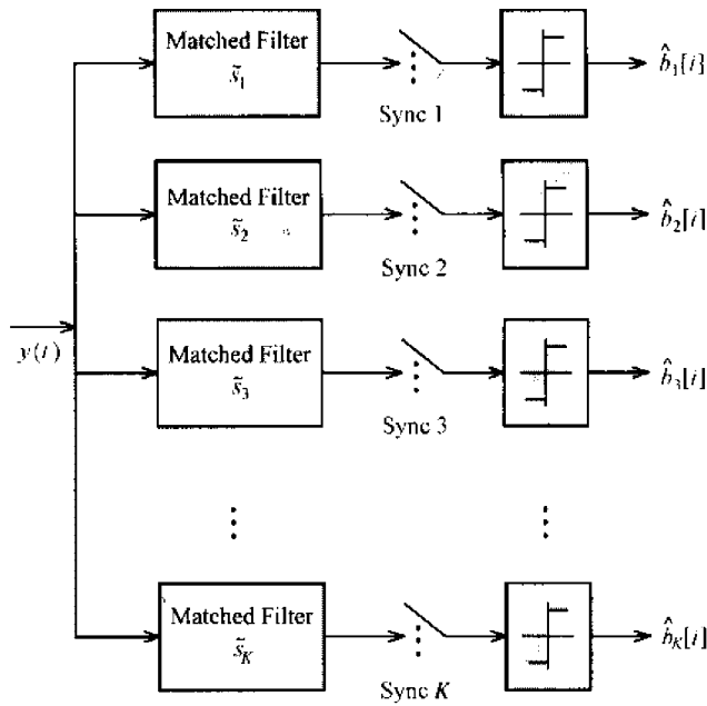
FIGURE 5.2. Modified matched filter bank for decorrelation.
