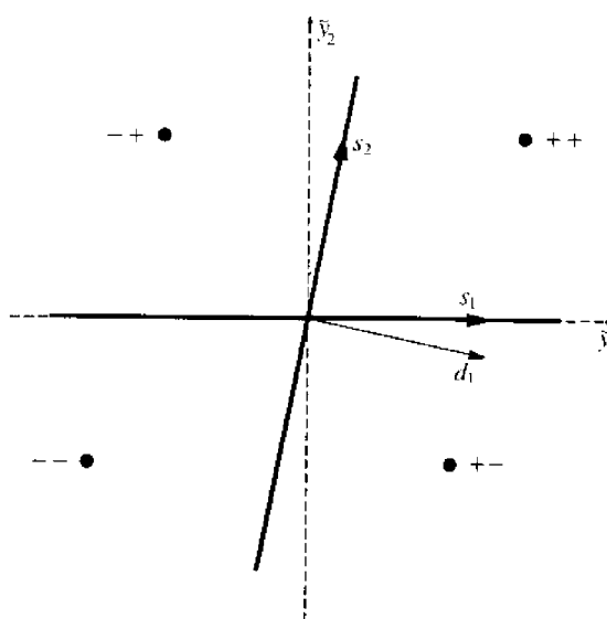
FIGURE 5.4. Decision regions of the two-user decorrelating detector; A_1 = A_2 .
