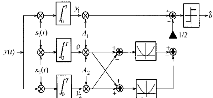
FIGURE 4.4. Minimum bit-error-rate detector for user 1 with one synchronous interferer.
