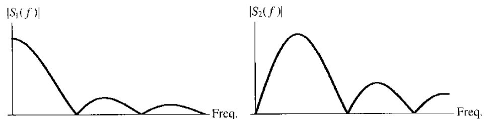
FIGURE 1.5. Fourier transforms (magnitude, f > 0 ) of waveforms in Figure 1.4.
