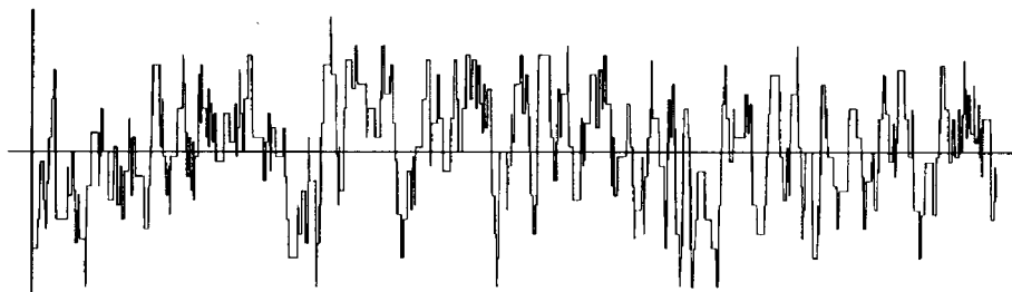
FIGURE 2.7. Noiseless sum of six modulated direct-sequence waveforms with N = 63 .
