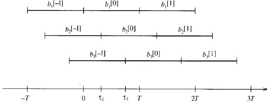
FIGURE 2.2. Bit epochs for K = 3 , M = 1 .
