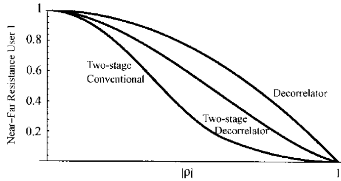
FIGURE 7.22. Near-far resistance of two-stage detectors with conventional and decorrelating first stage for synchronous users.
