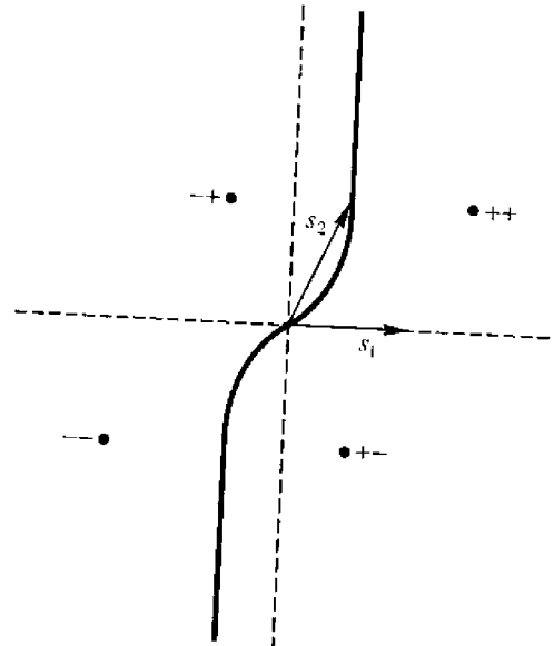
FIGURE 4.5. Decision regions of minimum bit-error-rate detector for user 1. A_1 = A_2 , \rho = 0.2 .
