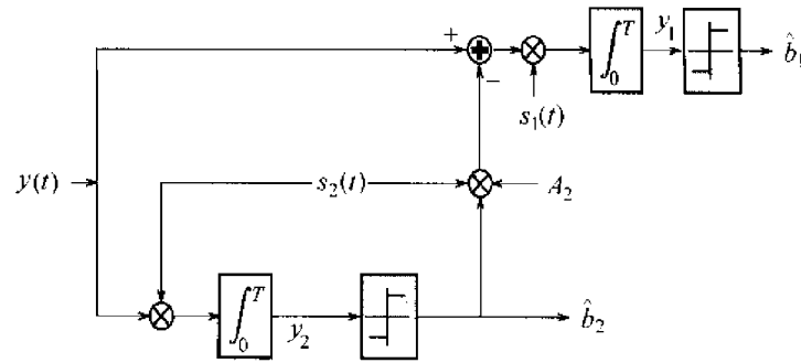
FIGURE 7.1. Successive cancellation for two synchronous users.
