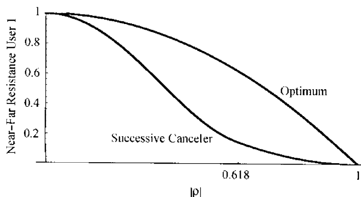
FIGURE 7.11. Near-far resistance for synchronous as a function crosscorrelati
