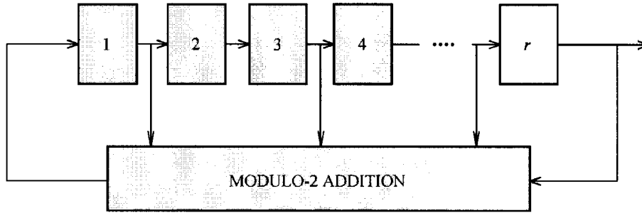
FIGURE 2.8. Generation of pseudonoise sequence with a feedback shift register.
