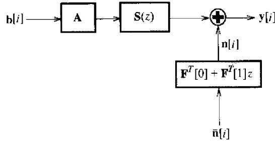
FIGURE 2.16. K-dimensional channel of matched filter outputs for asynchronous CDMA channel.
