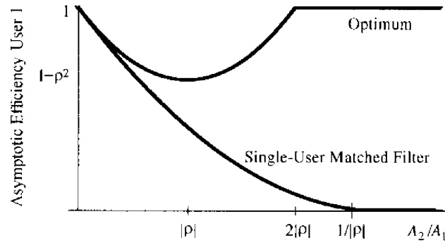
FIGURE 4.12. Optimum and single-user asymptotic multiuser efficiencies for two synchronous users.
