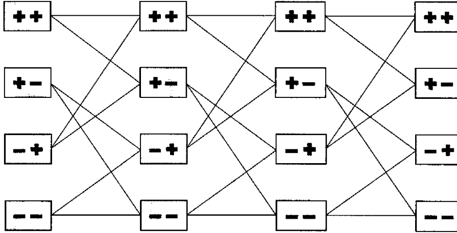
FIGURE 4.9. Trellis diagram for three-user asynchronous channel.
