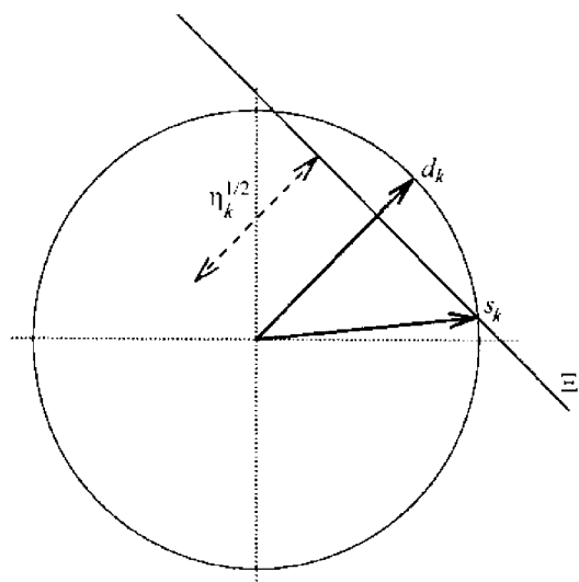
FIGURE 5.11. Optimality of decorrelating detector near-far resistance.
