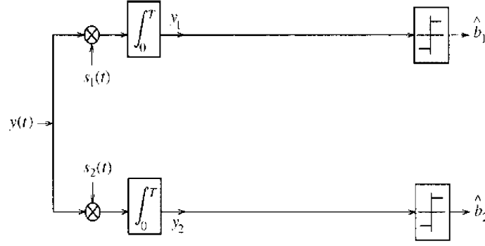
FIGURE 3.6. Bank of single-user matched filters ( K = 2 ).
