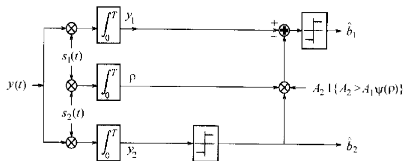
FIGURE 7.10. Modified successive cancellation two synchro users.
