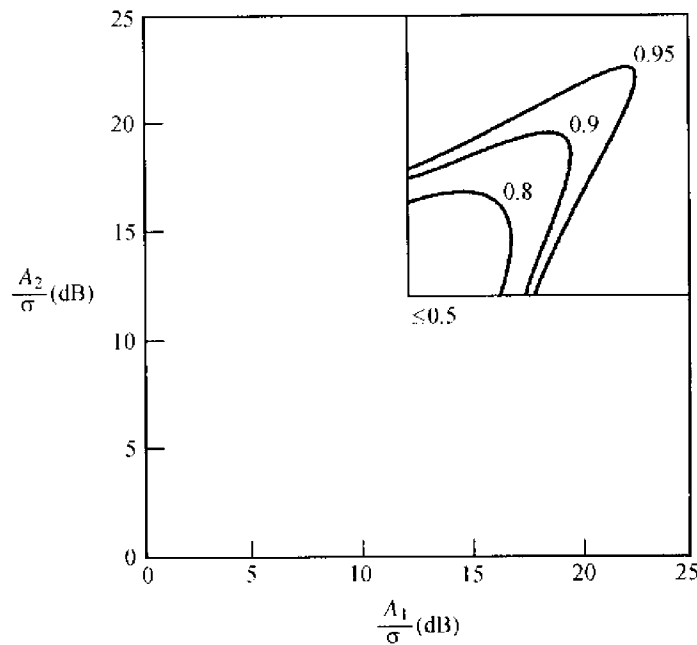
FIGURE 4.14. Signal-to-noise ratios necessary to achieve optimum bit-error-rate not higher than 3 \times 10^{-5} for both users.
