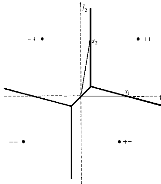
FIGURE 4.1. Decision regions of jointly optimum detector for A_1 = A_2 , \rho = 0.2 .
