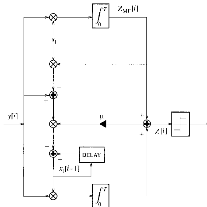
FIGURE 6.9. Blind adaptive multiuser dete
