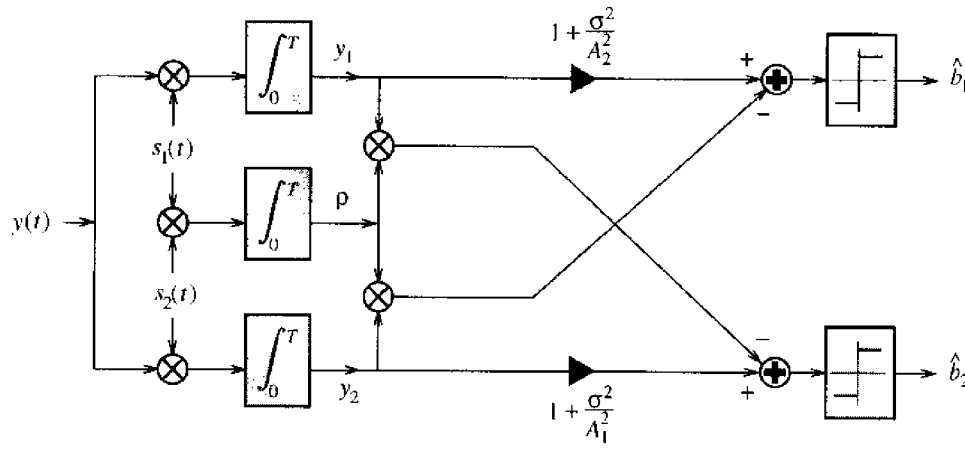
FIGURE 6.4. MMSE linear receiver for two synchronous users.
