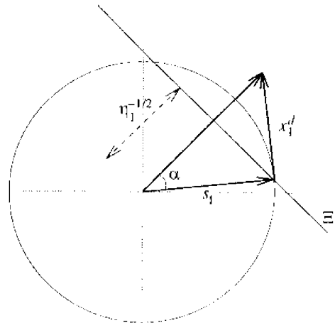
FIGURE 6.8. Decorrelating detector in canonical form
