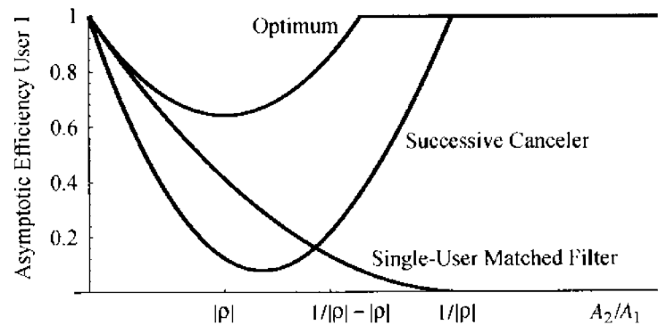
FIGURE 7.9. Asymptotic efficiencies for synchronous users; |\rho| = 0.6 .
