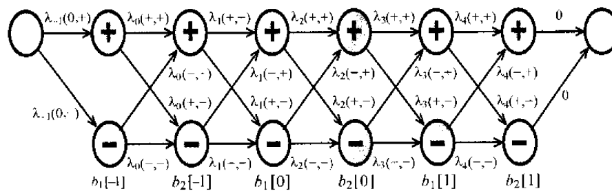
FIGURE 4.8. Trellis diagram for two asynchronous users; M = 1 .
