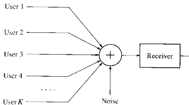
FIGURE 1.1. Multiaccess communication
