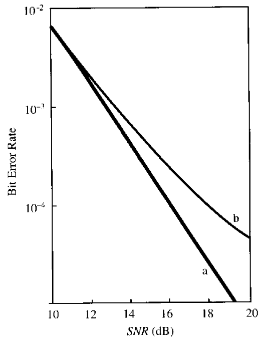
FIGURE 3.14. Bit-error-rate of the single-user matched filter with 10 equal-energy users and identical crosscorrelations \rho_{kl} = 0.08 ; (a) exact, (b) Gaussian approximation.
