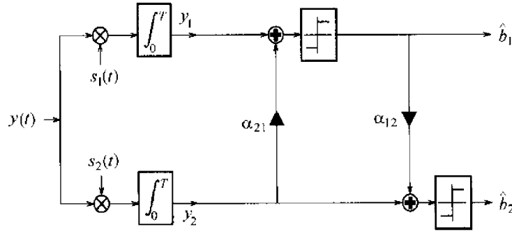
FIGURE 7.25. Two-user decision-feedback detector.
