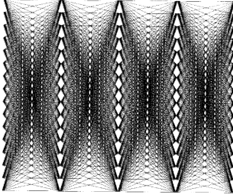
FIGURE 4.19. Trellis for a 4-user channel using the decomposition in Problem 4.15.
