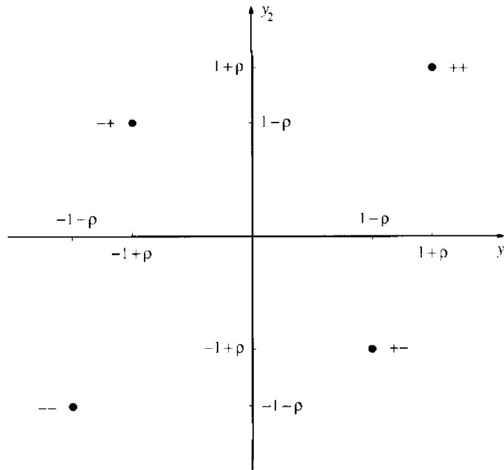
FIGURE 3.10. Decision regions in the two-dimensional space of matched filter outputs.
