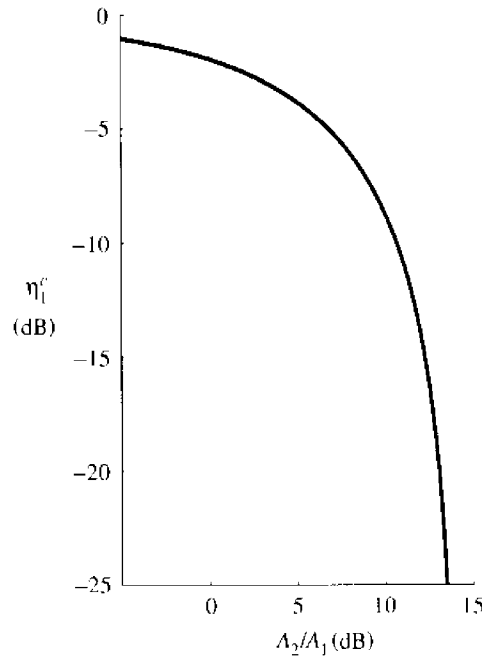
FIGURE 3.17. Asymptotic multiuser efficiency of conventional detector as a function of the amplitude of the interferer; \rho = 0.2 (log-log plot).
