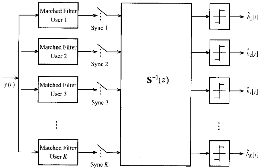
FIGURE 5.5. Asynchronous decorrelating detector.
