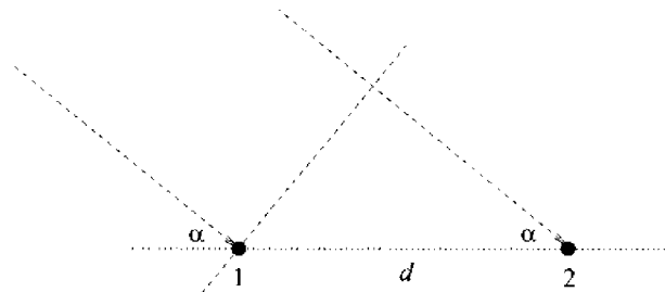
FIGURE 2.13. Two-element array.
