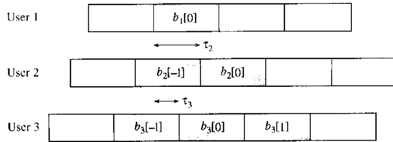
FIG 7.7. Timing window of users for demodulation of 1.
