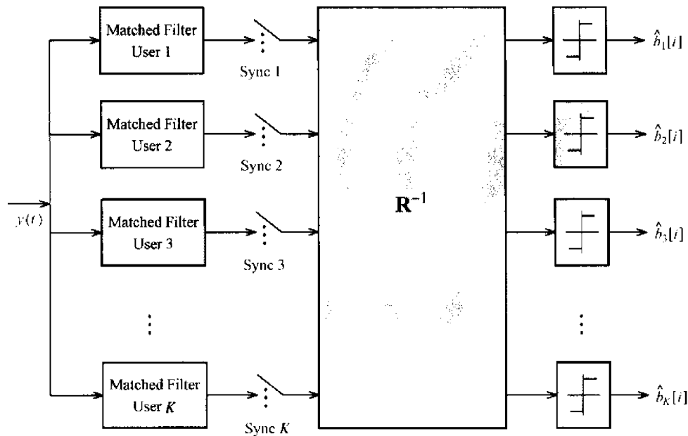
FIGURE 5.1. Decorrelating detector for the synchronous channel.
