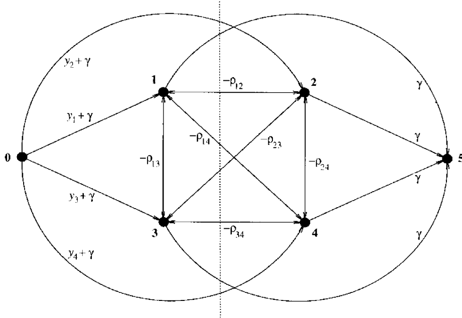
FIGURE 4.6. Directed graph for maximum-likelihood detection in the special case of four users with unit amplitudes.
