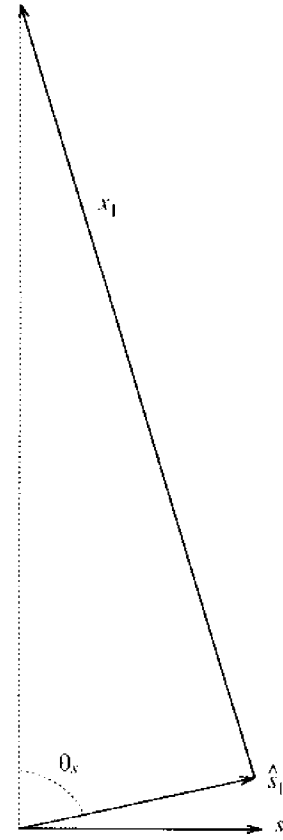
FIGURE 6.10. Complete desired-signal cancellation w mismatch.
