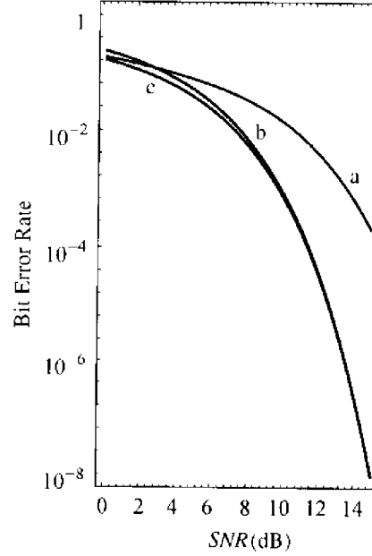
FIGURE 4.11. Bit-error-rate in a two-user channel with \rho = 0.4 , A_1 = A_2 : (a) single-user matched filter, (b) maximum-likelihood upper bound to minimum bit-error-rate, (c) genie lower bound to minimum bit-error-rate.
