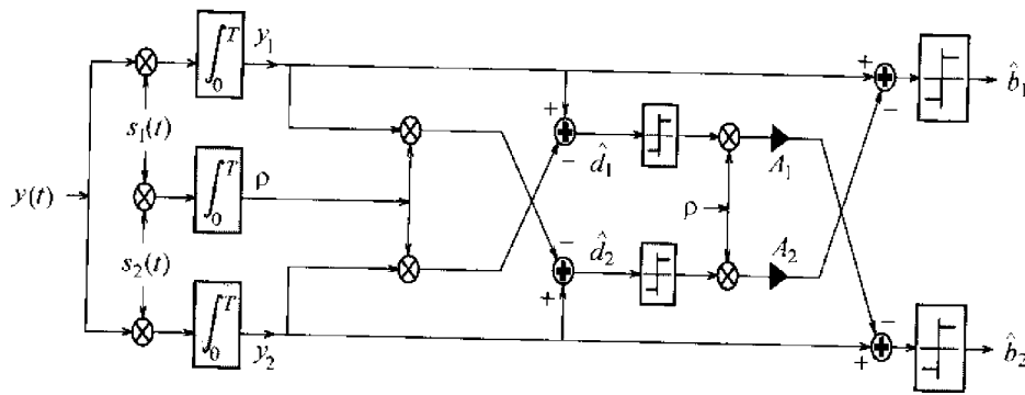
FIGURE 7.18. Two-stage detector with decorrelating first stage.
