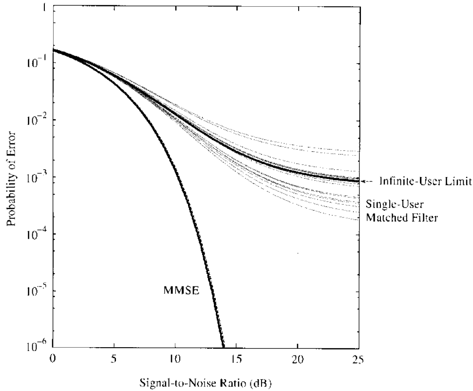
FIGURE 6.7. Bit-error-rate with 100 equal-power users and random direct sequence signatures with N = 1,000 .
