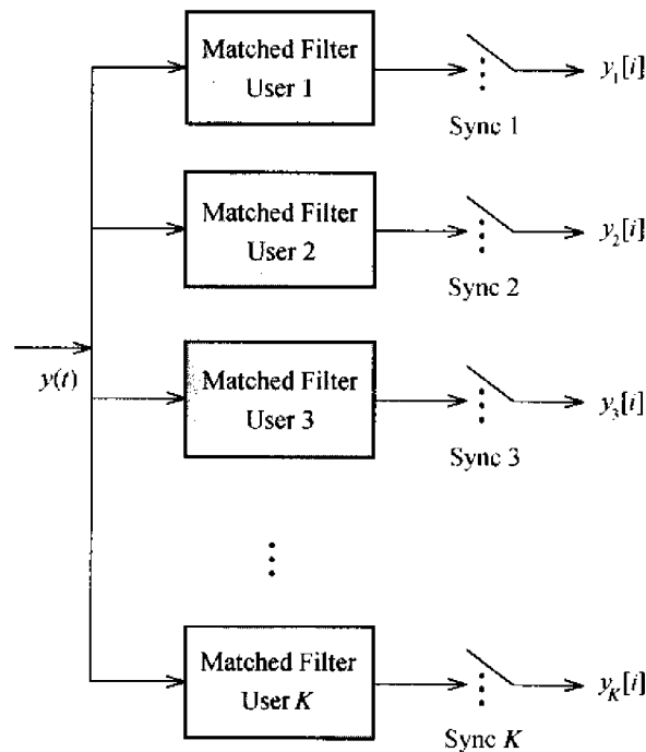
FIGURE 2.15. Discrete-time K -dimensional vector of matched filter outputs.
