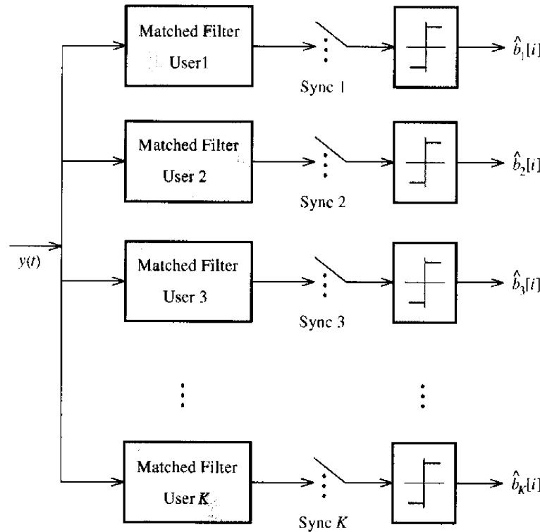
FIGURE 3.5. Bank of single-user matched filters.
