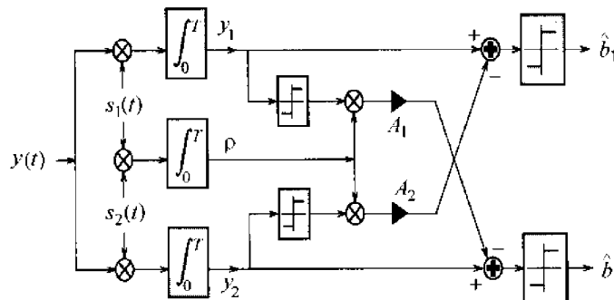
FIGURE 7.14. Multistage detector for two interfering users
