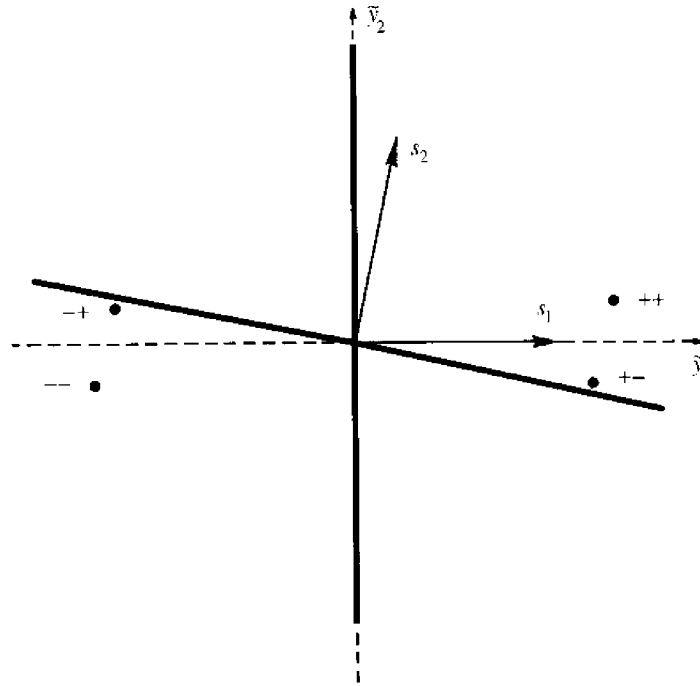
FIGURE 3.13. Decision regions of matched filter detector (orthogonal space); A_1 = 6A_2 .
