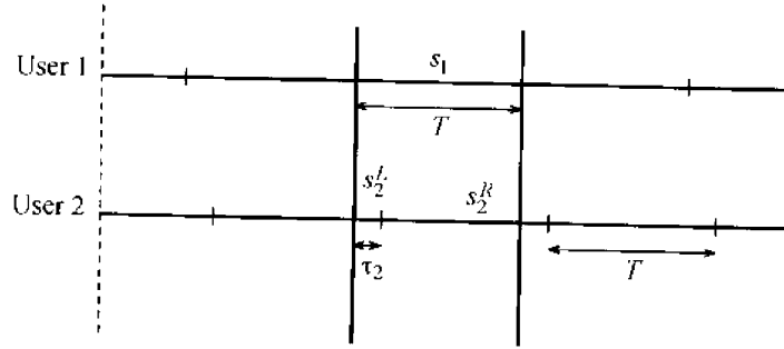
FIGURE 5.6. One-shot approach to demodulation in asynchronous two-user channel.
