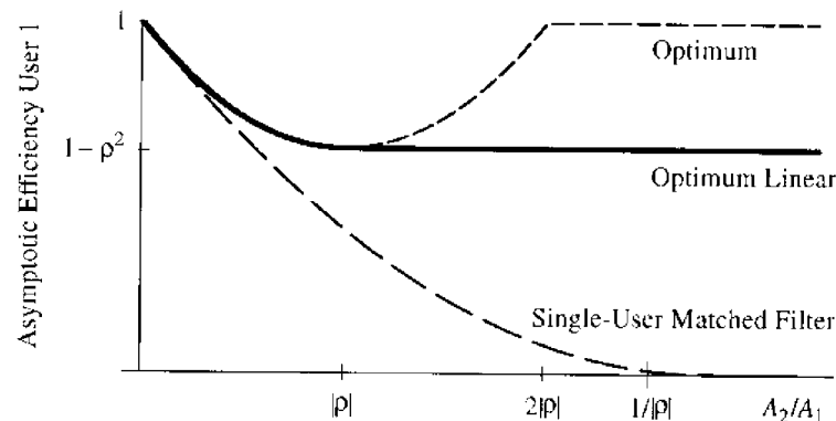
FIGURE 6.2. Asymptotic multiuser efficiencies for two synchronous users.
