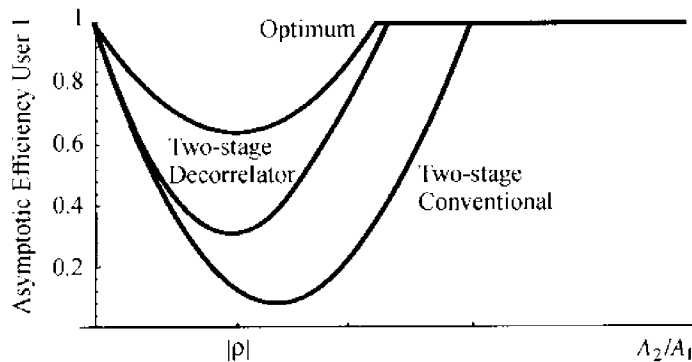
RE 7.21. Asymptotic user efficiencies for synchronous ; |\rho| = 0.6 .
