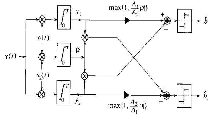
FIGURE 6.1. Linear detector that maximizes asymptotic efficiency for the two-user synchronous channel.
