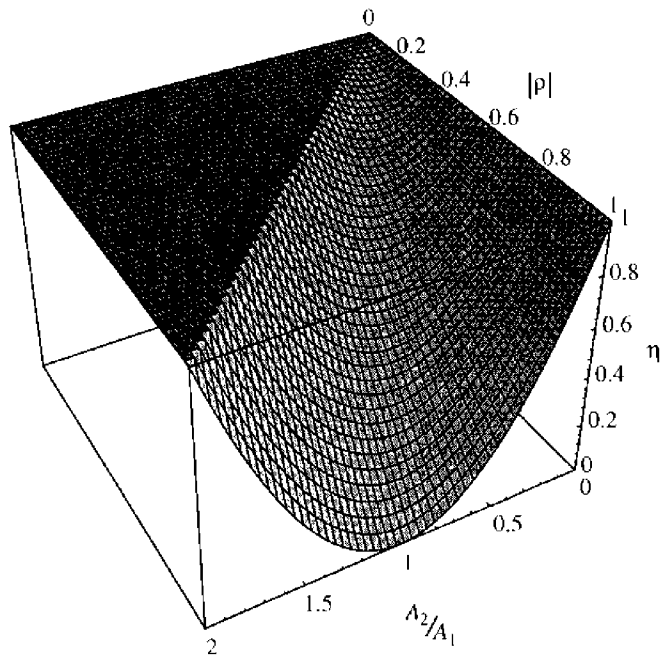
FIGURE 4.13. Optimum asymptotic multiuser efficiency as a function of |\rho| and relative amplitude interferer.
