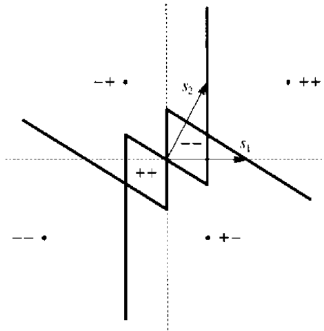
FIGURE 7.15. Decision region of two-stage detector with A_1 = 1 , A_2 =
