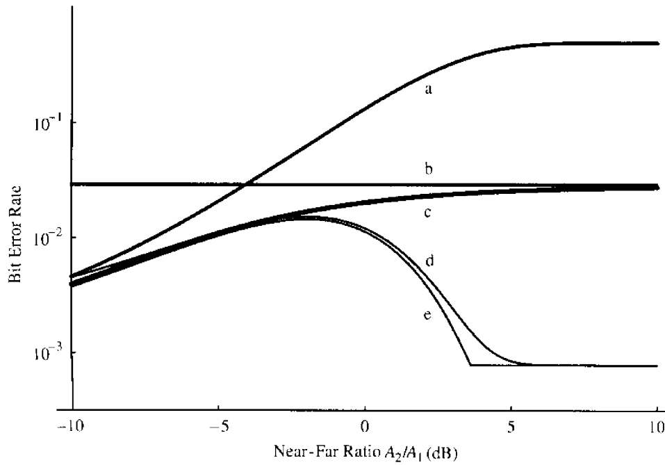
FIGURE 6.5. Bit-error-rate with two users and crosscorrelation \rho = 0.8 : (a) single-user matched filter; (b) decorrelator; (c) MMSE; (d) minimum (upper bound); (e) minimum (lower bound).
