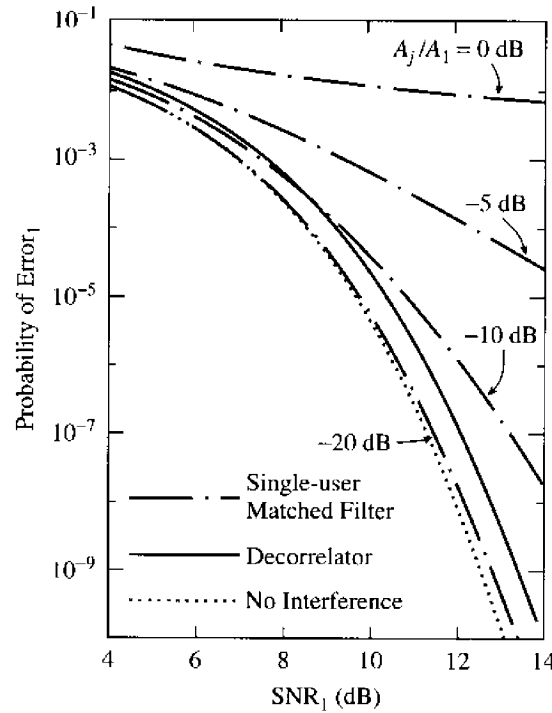
FIGURE 5.12. Bit-error-rate of decorrelating detector and single-user matched filter detector. Five equal-energy interferers.
