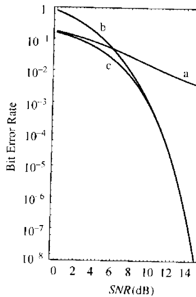
FIGURE 4.16. Bit-error-rate in a fifteen-user channel with equal-power users and \rho_{kl} = 0.09 ; (a) conventional, (b) maximum-likelihood upper bound to minimum bit-error-rate, (c) lower bound to minimum bit-error-rate.
