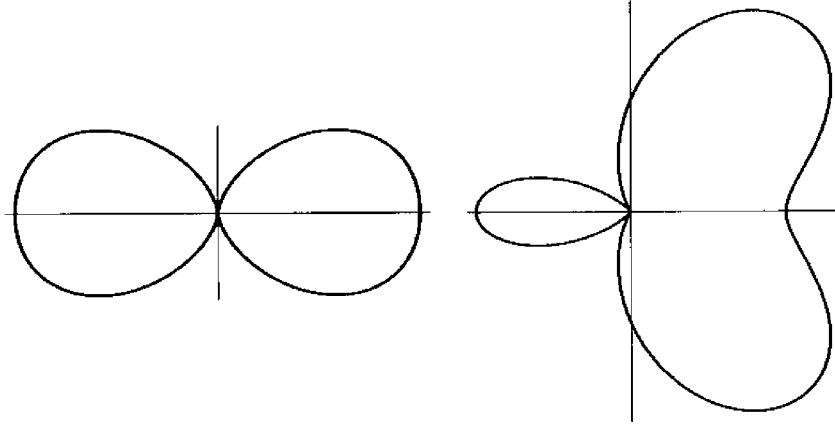
FIGURE 2.14. Two-element array radiation patterns with equal gains and phase offsets of \varphi = \pi (left) and \varphi = \pi/2 (right).
