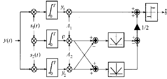
FIGURE 4.3. Maximum-likelihood detection for user 1 with one synchronous interferer.
