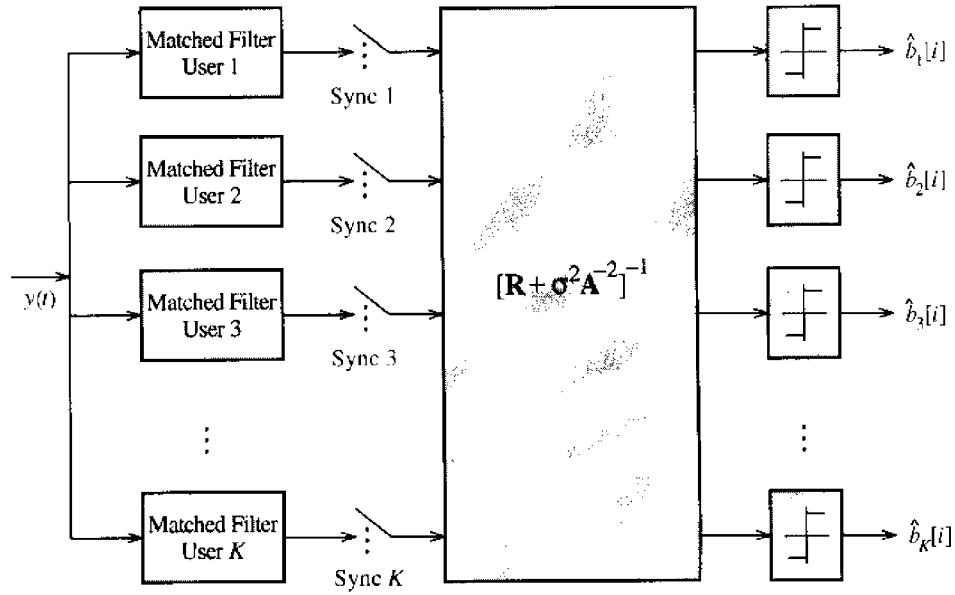
FIGURE 6.3. MMSE linear detector for the synchronous channel.
