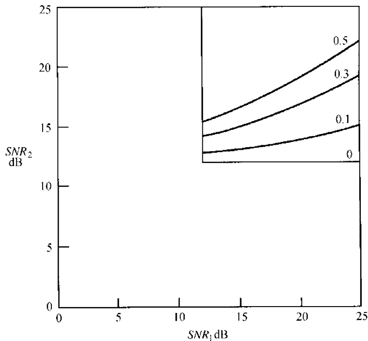
FIGURE 7.12. Signal-to-noise ratio necessary for successive cancellation to give error-rate not greater than 10^{-5} for both users. Shown for \rho = 0.3, 0.5 .
