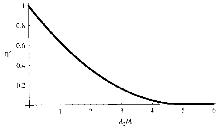
FIGURE 3.16. Asymptotic multiuser efficiency of conventional detector as a function of the amplitude of the interferer; \rho = 0.2 (linear plot).
