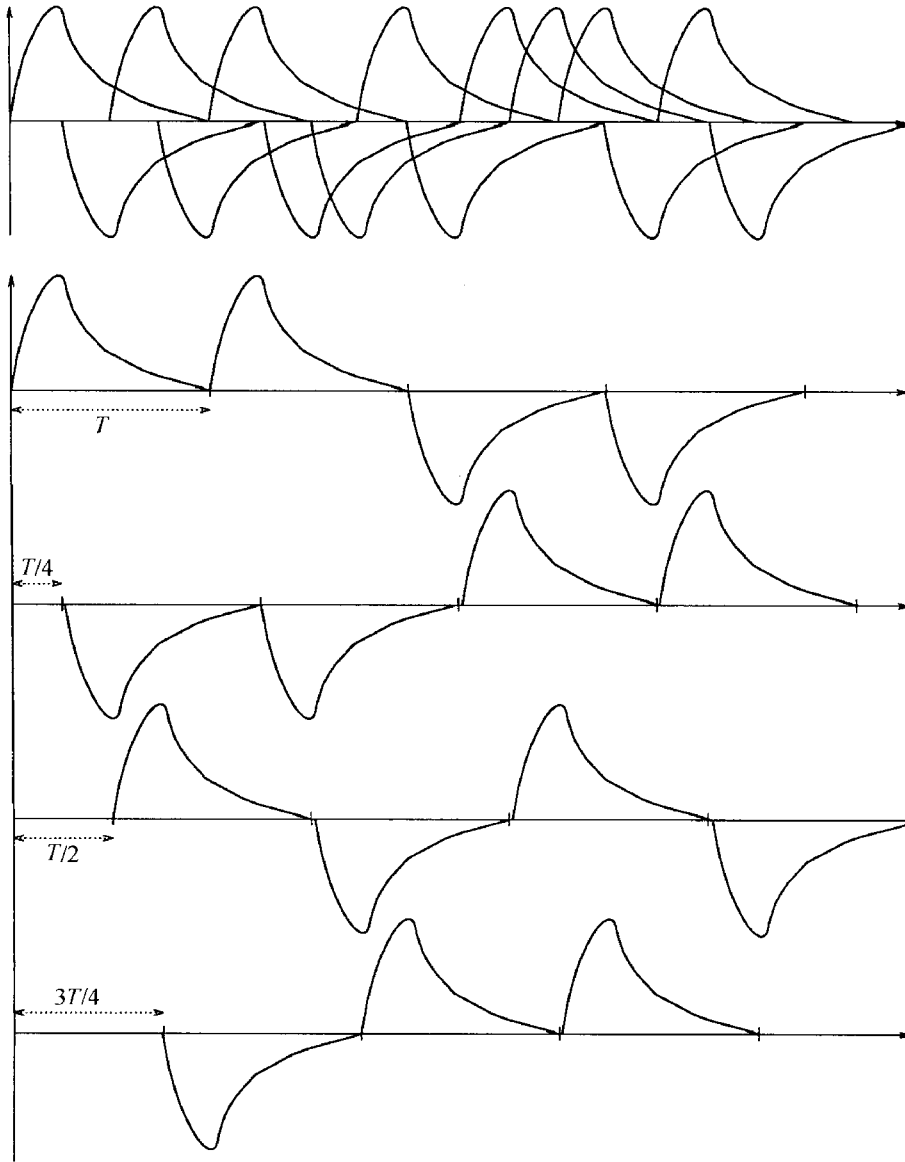
FIGURE 2.3. Intersymbol interference as an asynchronous CDMA channel.
