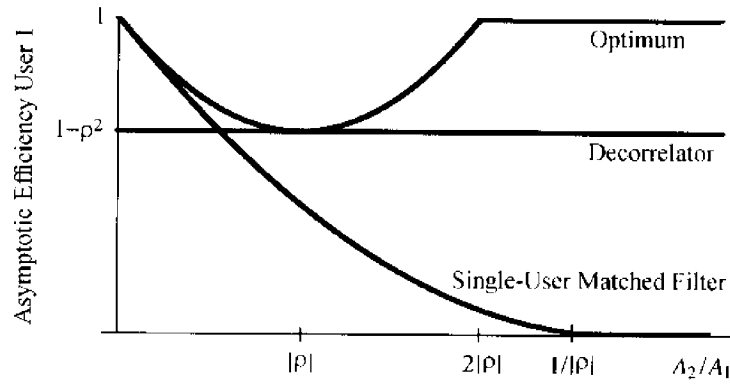
FIGURE 5.8. Asymptotic multiuser efficiencies for two synchronous users.
