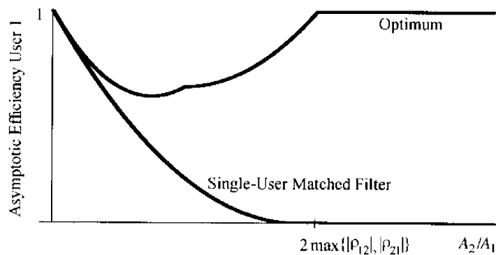
FIGURE 4.17. Optimum and single-user matched-filter asymptotic multiuser efficiencies as functions of the amplitude of the interferer.
