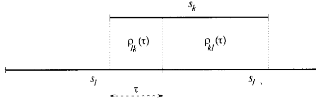
FIGURE 2.4. Definition of asynchronous crosscorrelations ( k < l ).
