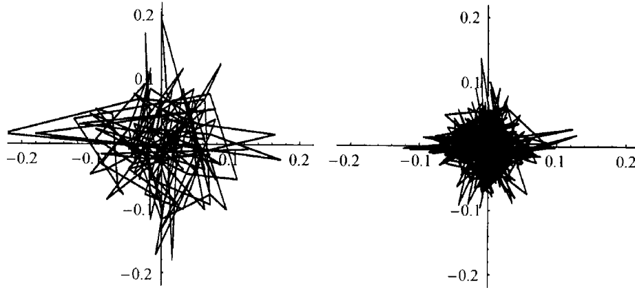
FIGURE 2.10. Locus of crosscorrelations (\rho_{12}, \rho_{21}) for N = 128 (left) and N = 512 (right) with rectangular chips.
