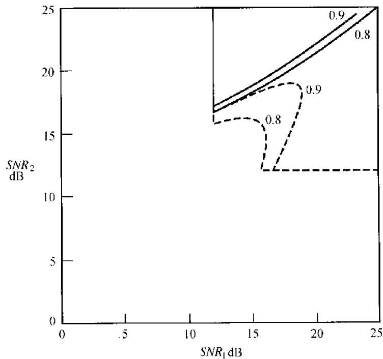
FIGURE 7.13. Signal-to-noise ratio necessary for successive cancellation to give error-rate not greater than 10^{-5} for both users. Shown for \rho = 0.8, 0.9 , compared with the optimal solutions (dashed).
