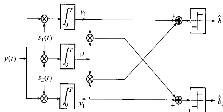
FIGURE 5.3. Decorrelating receiver for two synchronous users.
