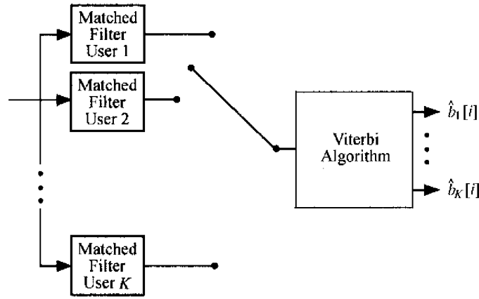
FIGURE 4.10. Optimum multiuser detector for asynchronous CDMA.
