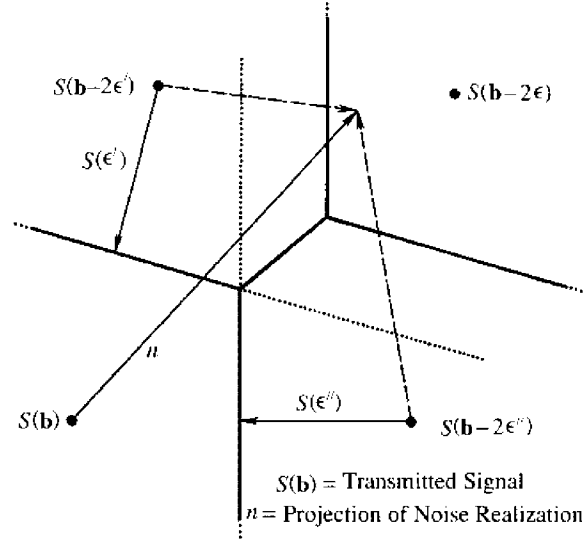
FIGURE 4.15. If \epsilon is decomposable into \epsilon' and \epsilon'' , and \mathbf{b} - 2\epsilon is the most likely vector, then both \mathbf{b} - 2\epsilon' and \mathbf{b} - 2\epsilon'' are more likely than \mathbf{b} .
