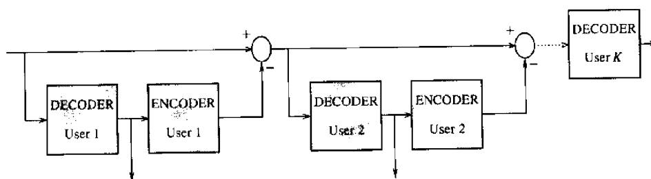
FIGURE 1.8. Successive decoding.
