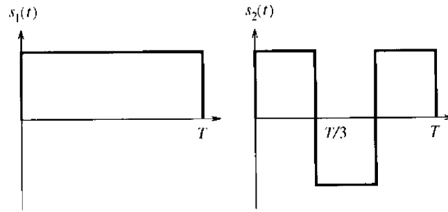
FIGURE 2.17. Direct sequence signature waveforms with N = 3 .
