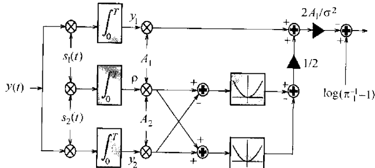
FIGURE 4.18. Computation of the a posteriori probability P[b_1 = +1|y] from the a priori probability \pi_1 = P[b_1 = +1] .
