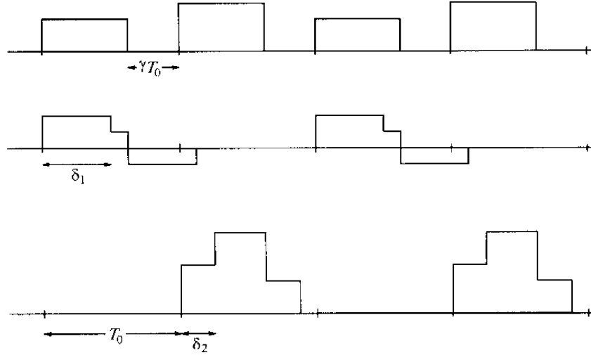
FIGURE 2.18. TDMA signals subject to multipath. K = 2 , \alpha_1 = -0.5 , \alpha_2 = 2/3 , \gamma = 3/8 .
