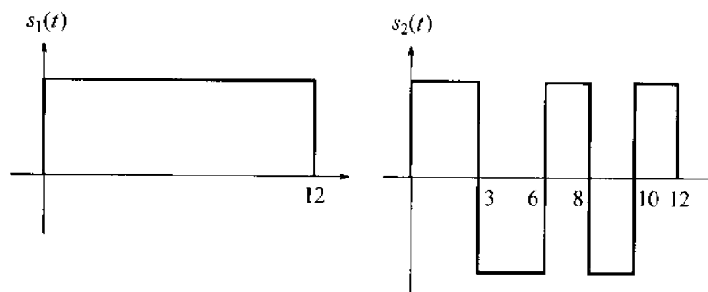
FIGURE 5.13. Signature waveforms for Problem 5.20.
