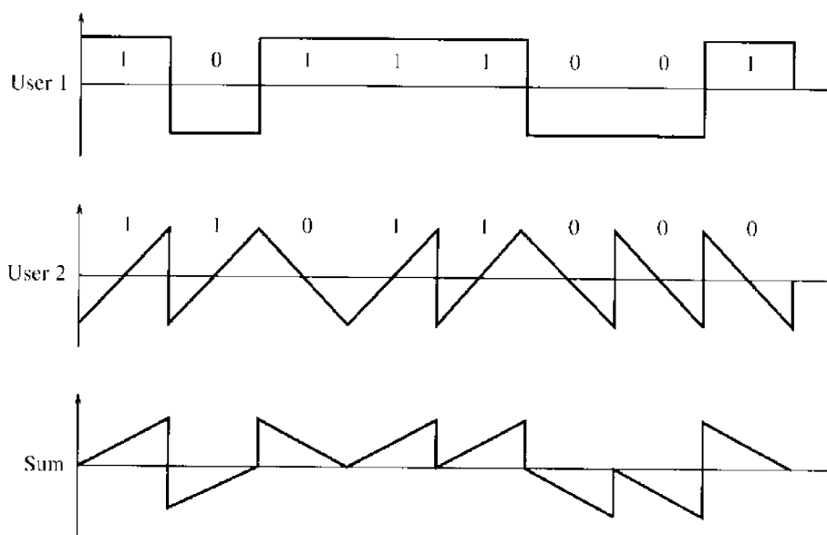
FIGURE 1.6. Synchronous antipodal modulation of orthogonal signals.
