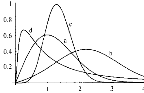
FIGURE 2.12. Probability density functions: (a) Rayleigh; (b) Rice ( d = 2 ); (c) Nakagami ( d = 3 ); (d) log-normal ( \sigma_p = 10 ).
