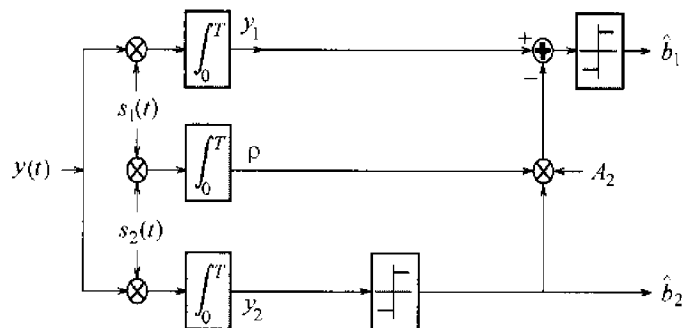
FIGURE 7.2. Equivalent implementation of successive cancellation for two synchronous users.
