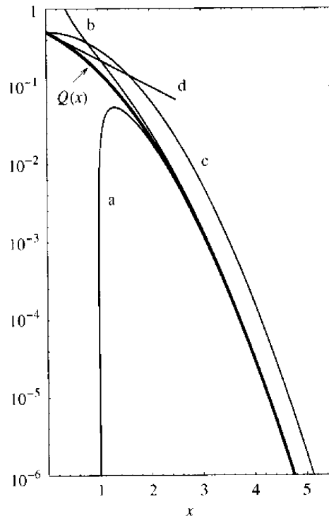
FIGURE 3.4. Log-linear plot of Q(x) and its bounds: (a) (3.34), (b) (3.35), (c) (3.37), and (d) (3.38).
