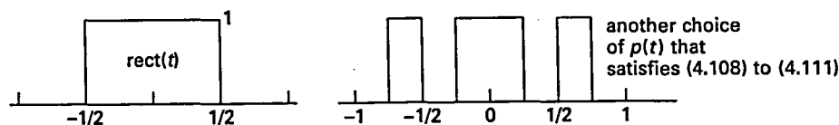
Figure 4.12. Two functions that each satisfy (4.108)–(4.111)
