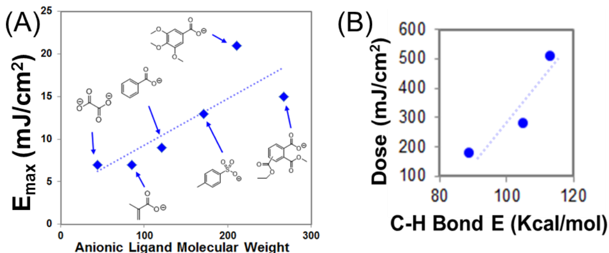
Figure 3. Sn-12 oxocluster reactivity served as basis for further experiments. (A) Linear relationship between molecular weight ( \text{g}/\text{mol} ) and sensitivity ( \text{mJ}/\text{cm}^2 ) and (B) Linear relationship between bond strength and sensitivity.
