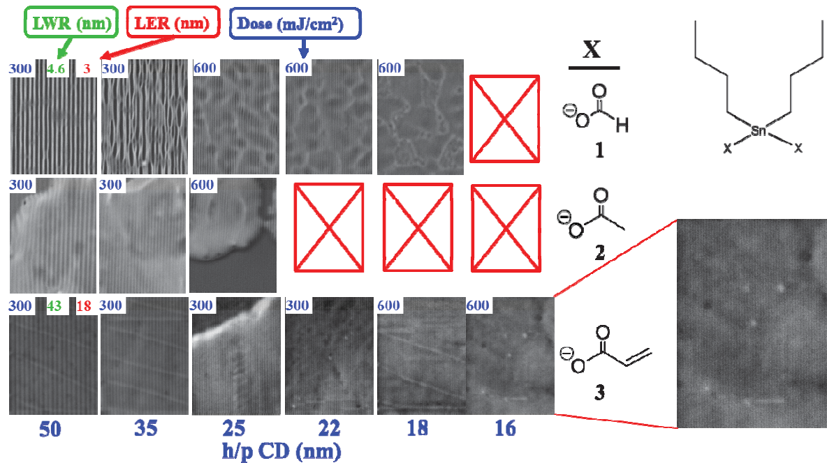
Figure 5. Dense lines patterning capabilities of dibutyl tin dicarboxylates. All of the films exhibited poor film quality after development.
