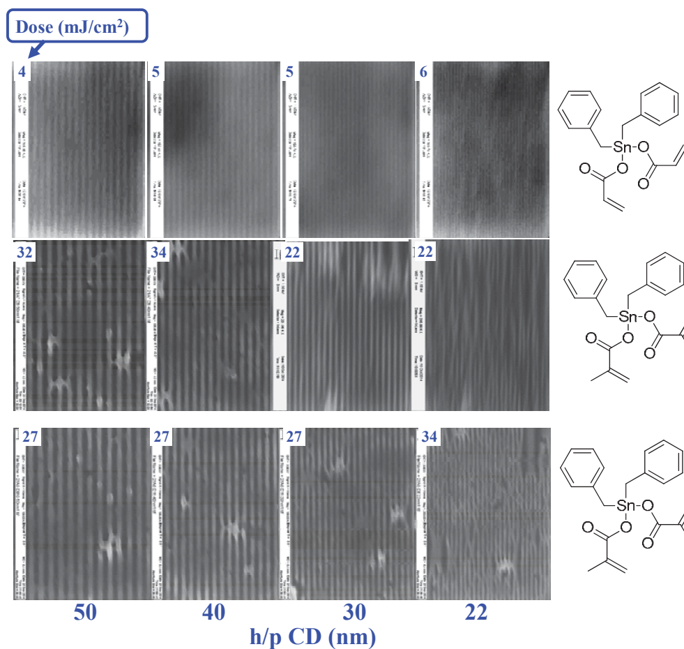
Figure 9. Dibenzyl tin acrylates displayed much higher photospeeds at a cost of resolution and LER.
