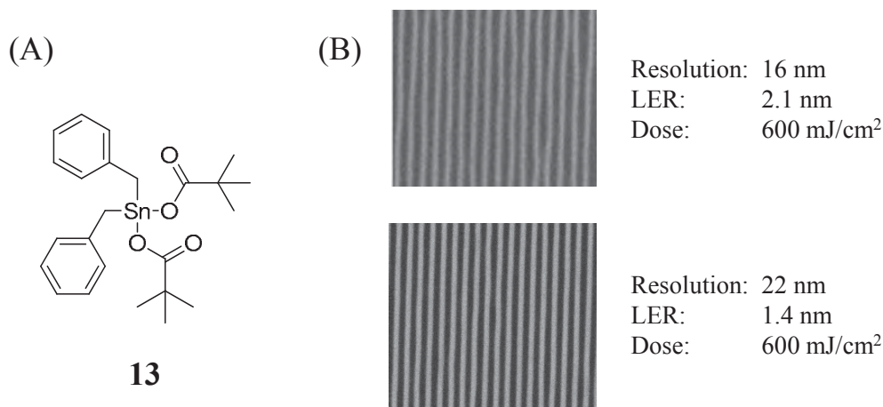
Figure 1. (A) Structure of Compound 13 , (C_6H_5CH_2)_2Sn(O_2C(C(CH_3)_3))_2 . (B) Dense line patterning capabilities of compound 13 exhibiting low LER.
