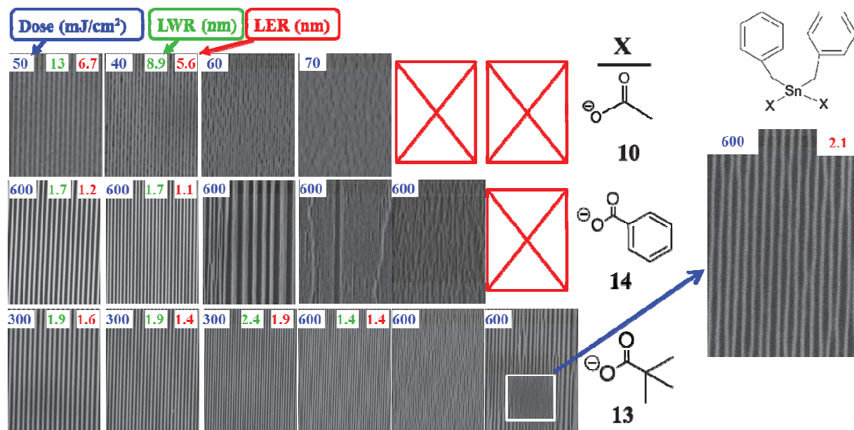
Figure 7. Dense lines patterning capabilities dibenzyl tin dicarboxylates. These resists achieved the highest resolution and lowest LER of any metal based resist evaluated by our group.
