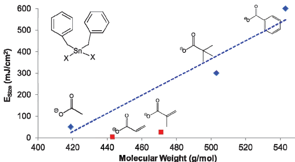
Figure 3. Patterning shows the same linear dependence with a significant deviation when analyzing acrylate based resists.
