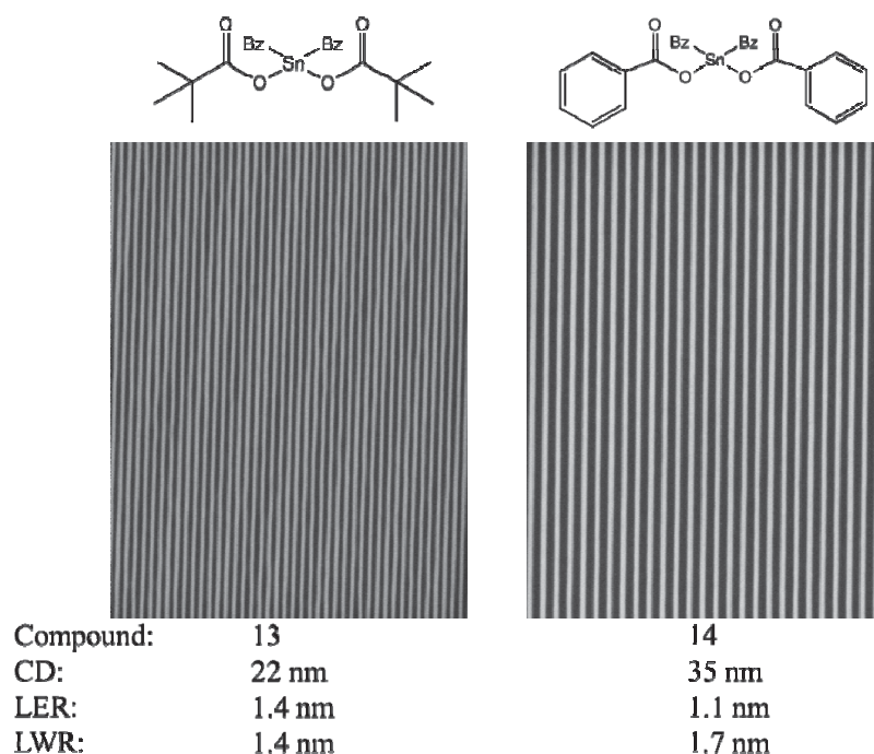
Figure 8. Compounds 13 and 14 display high resolution patterning with extremely low LER.
