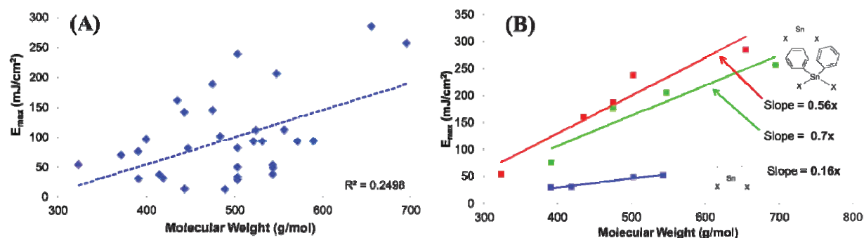
Figure 2. (A) Comparing a wide variety of organotin carboxylates shows little correlation of data, however, (B) strong correlations exist when comparing a particular family of compounds.
