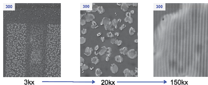
Figure 6. Strange patterning phenomenon of compound (C_4H_9)_2Sn(O_2CCH_3)_2 ( 2 ). Each island shows patterning with no patterning in the spaces.
