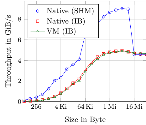
Figure 1: Throughput Overhead
