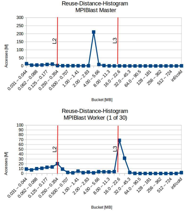
Figure 3: Reuse Distance Histogram for MPIBlast. Master (top) is distributing chunks of workload to workers (bottom) which all have the same histogram.
