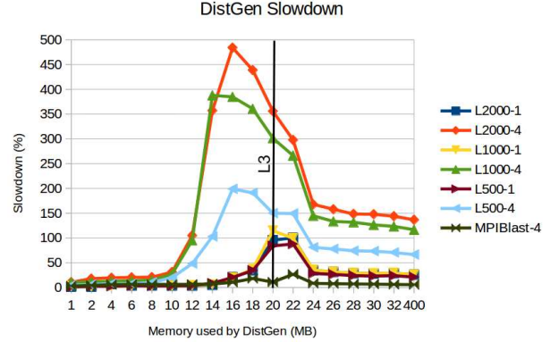
Figure 6: Slowdowns perceived by our micro-benchmark DistGen when running against various applications.
