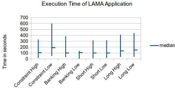
Figure 5: The runtime of the LAMA applications with different governors.
