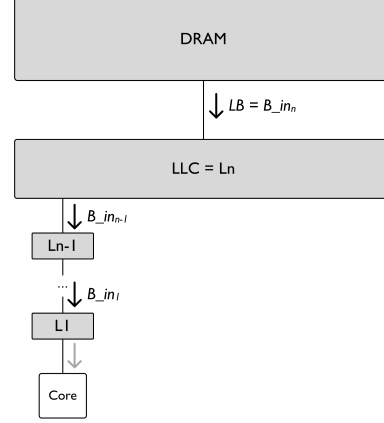
Figure 2: Inspected data flow in the memory hierarchy
