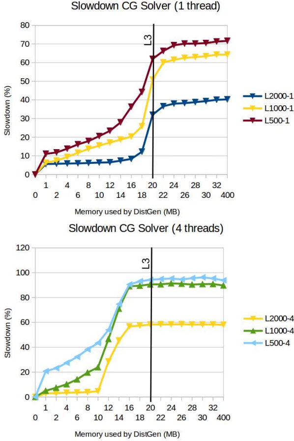
Figure 4: Slowdowns perceived by LAMA with 1 (top) and 4 threads (bottom), running against DistGen with 4 threads.
