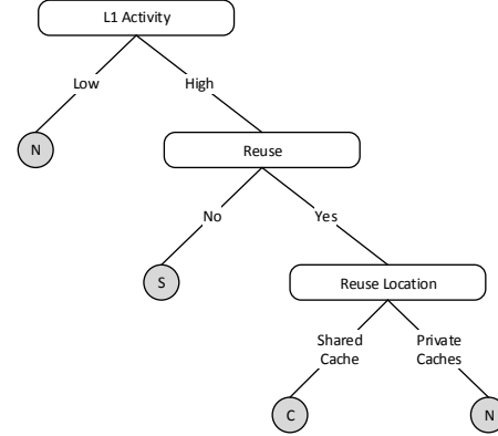
Figure 2: Inspected data flow in the memory hierarchy
