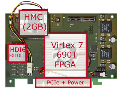
Fig. 2: Network Attached Memory (NAM) board.
