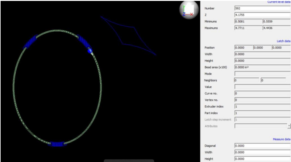
Ex. E (July 5, 2011, packed CMB file) at 16. As shown in layer 592, the blue lines indicate support material, and the green lines indicate part material. The blue diamond shape represents a layer of the purge tower, corresponding to a switch to the printing of support material on this layer.
