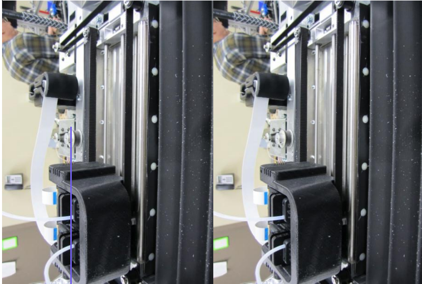
Ex. C (November 20, 2011, photograph showing Solo's print heads and deposition lines).
