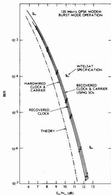
Fig. 29. BER performance for 120-Mbit/s modem.
