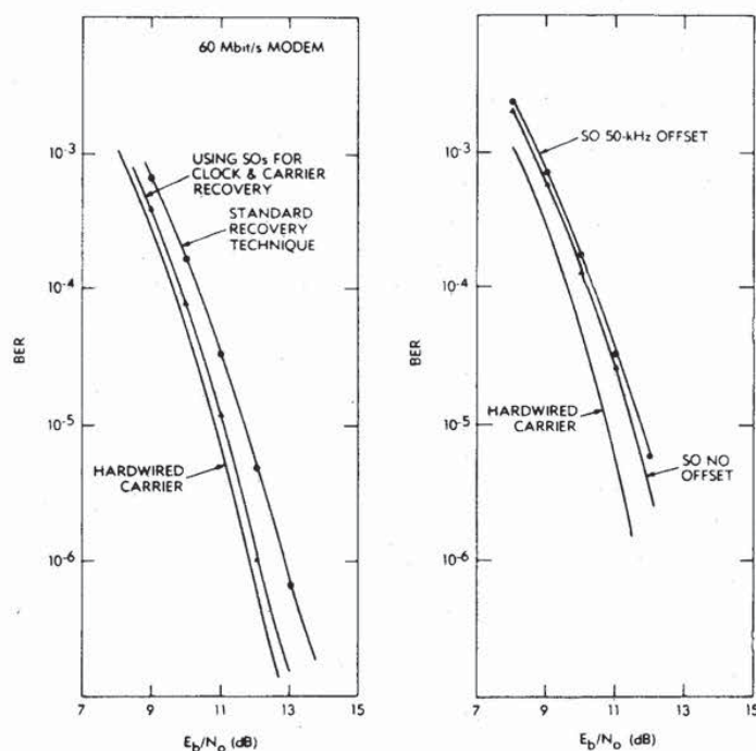
Fig. 28. BER performance of 60-Mbit/s modem.
