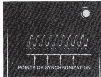
Fig. 14. Synchronization in a divide-by- 3/2 process.
