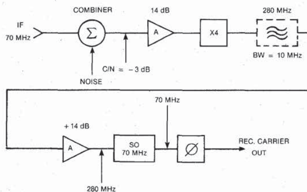
Fig. 26. SO carrier recovery network.
