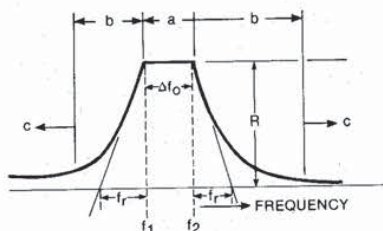
Fig. 5. Operation regions of an SO.
