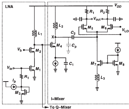
Fig. 2. LNA/mixer implementation.
