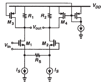
Fig. 5. Baseband amplifier.
