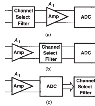
Fig. 4. Baseband processing.
