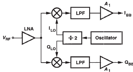
Fig. 1. Receiver architecture.
