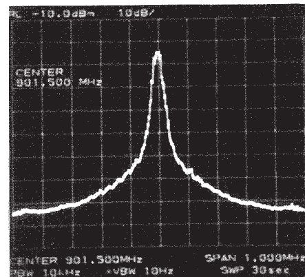
Fig. 6. LO divided output spectrum. (Horiz., 100 kHz/div.; Vert. 10 dB/div.; Resolution bandwidth, 10 kHz.)
