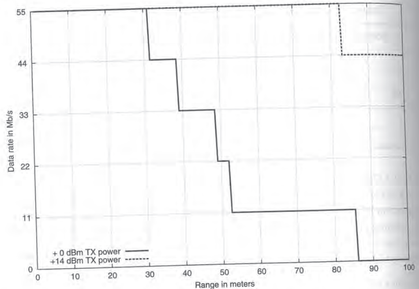
Figure 7–1: Rate vs. range for high and low power 802.15.3 2.4 GHz PHY
