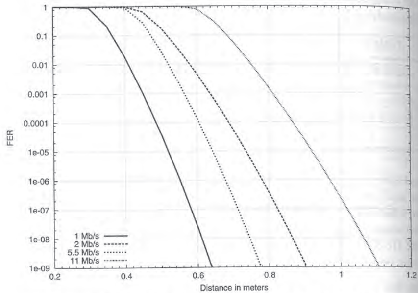
Figure 9-5: FER results for 802.11b with 802.15.3 as the interferer in the adjacent channel
