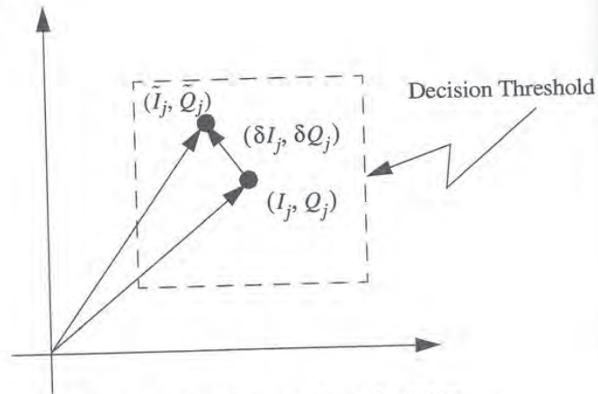
Figure 7-13: Error vector calculation
