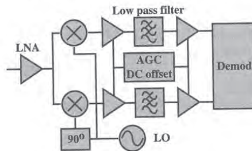
Figure 7-17: Direct conversion radio architecture
