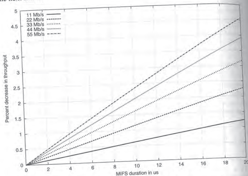
Figure 7-3: Percent throughput lost for each of the supported data rates at various MIFS durations
