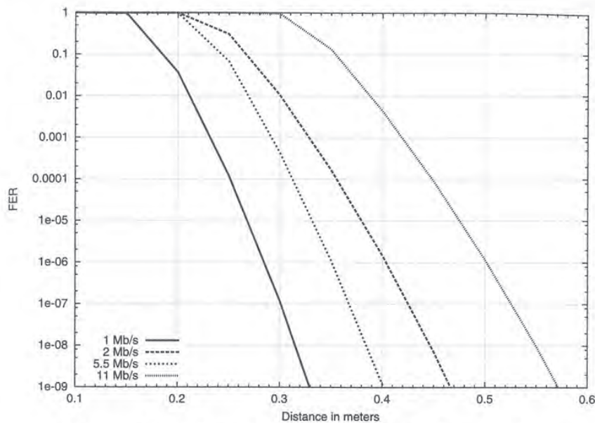
Figure 9-6: FER results for 802.11b with 802.15.3 as the interferer in the alternate channel
