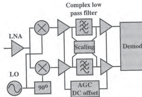
Figure 7-19: Low IF radio architecture
