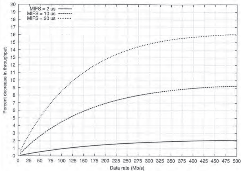
Figure 7-2: Percent throughput lost due to a non-zero MIFS
