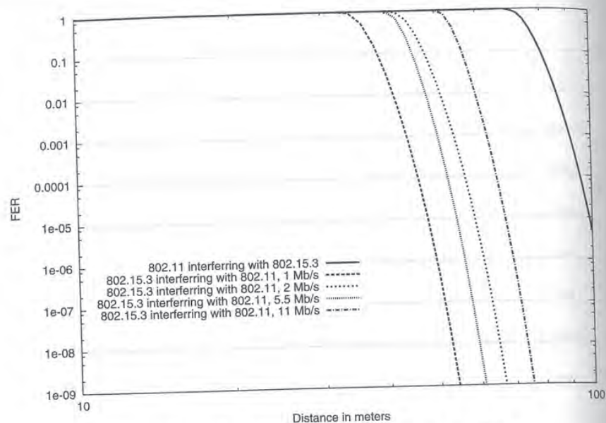
Figure 9-7: FER results for 802.11b and 802.15.3 co-channel interference
