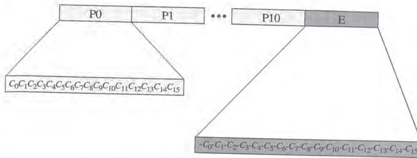
Figure 7-7: Physical layer preamble format
