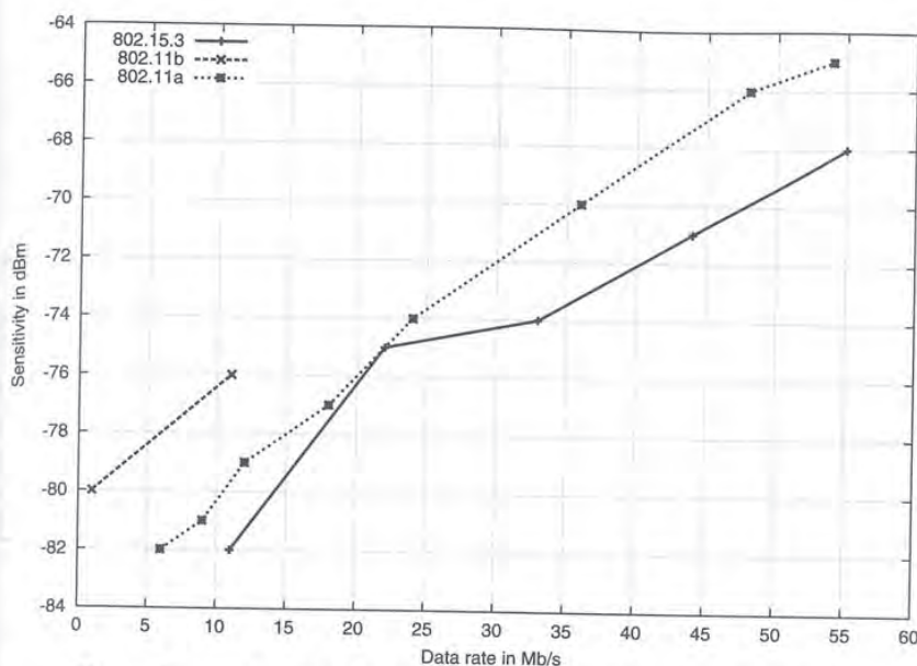
Figure 7-11: Comparison of receiver sensitivities for 802.11a, 802.11b, and 802.15.3
