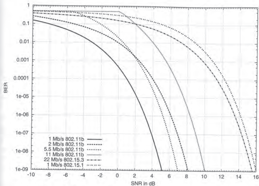
Figure 9-3: BER versus SNR for 802.11b, 802.15.3, and 802.15.1
