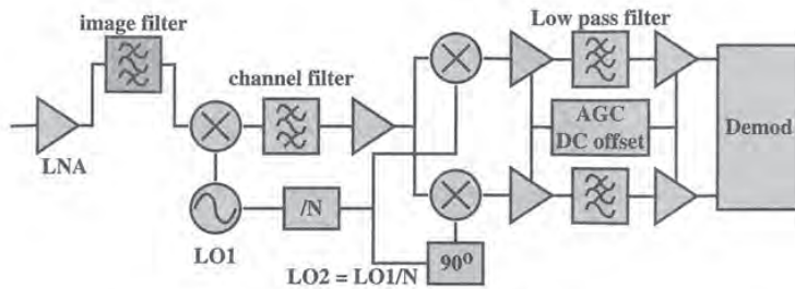
Figure 7-18: Walking IF radio architecture
