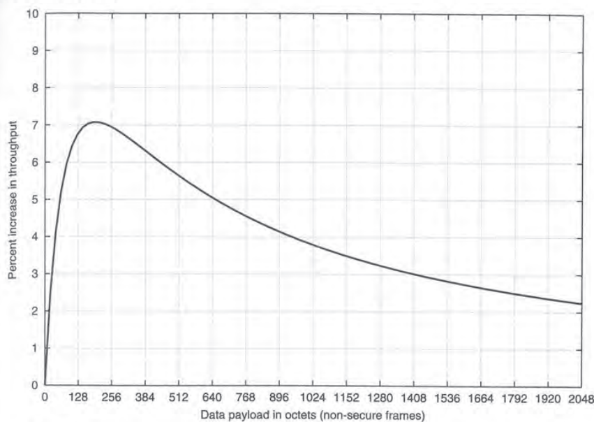
Figure 7-4: Percent throughput increase from changing the MIFS duration from 10 \mu s to 2 \mu s for various data payload sizes
