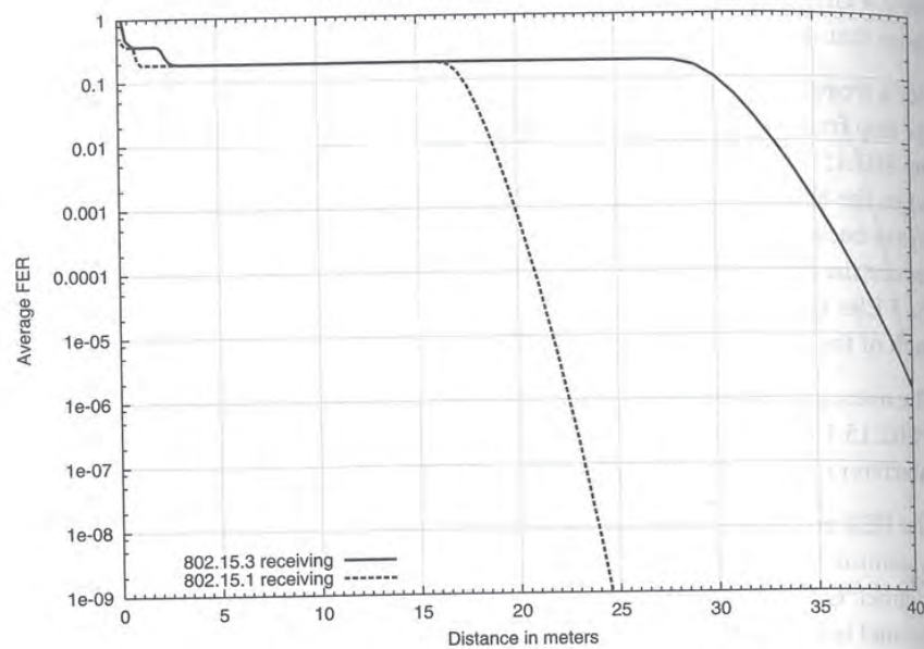
Figure 9-8: Average FER results for 802.15.1 and 802.15.3
