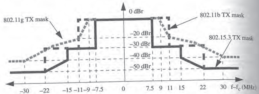
Figure 9-1: 802.15.3 and 802.11b transmit spectral mask
