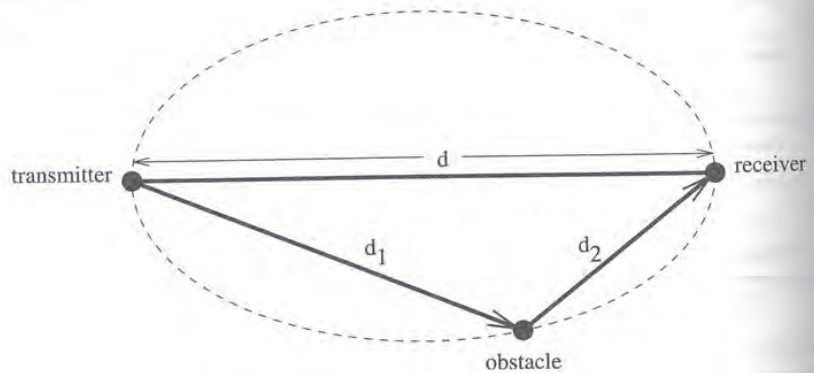
Figure 7-14: Geometry for two-ray multipath
