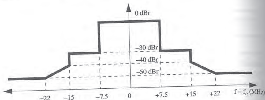
Figure 7-12: Transmit power spectral density mask
