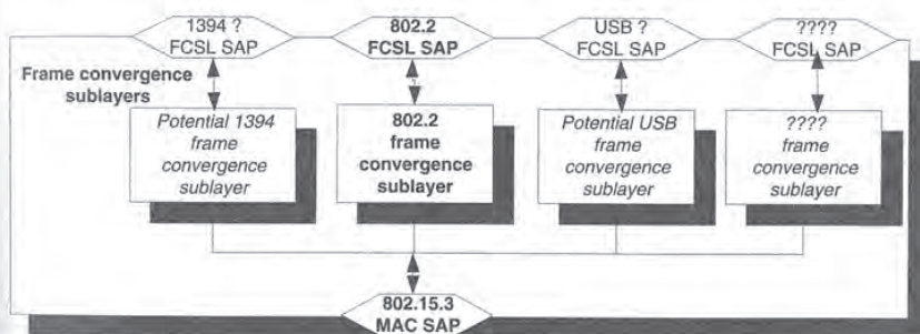
Figure 8-2: Frame convergence sublayer model
