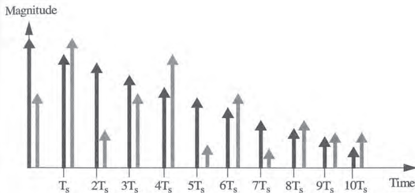
Figure 7-15: Channel impulse response used for 802.15.3 evaluation
