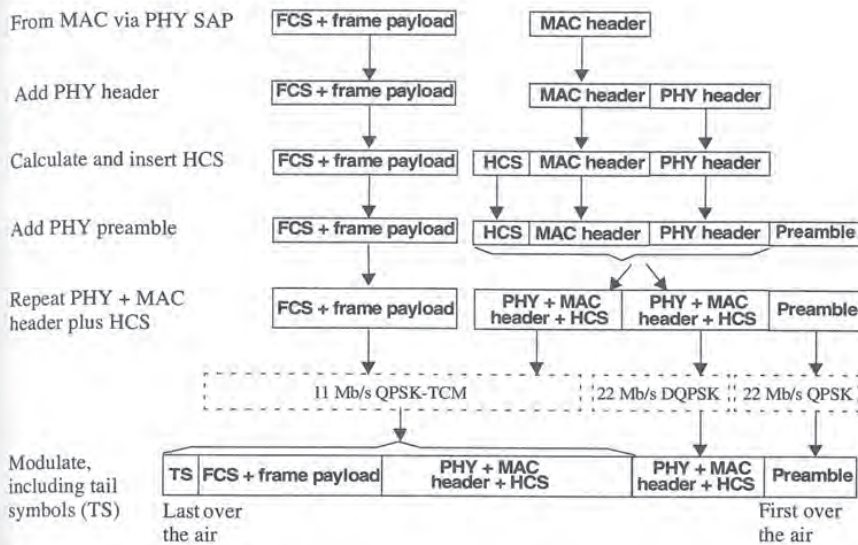
Figure 7-6: PHY frame formatting for 11-Mb/s mode
