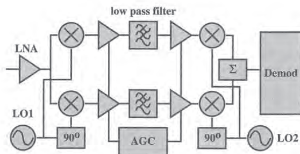
Figure 7-21: Low IF using the Weaver architecture
