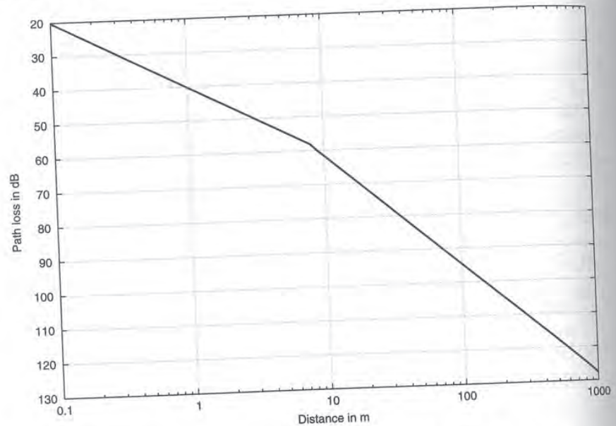
Figure 9-2: Path loss versus distance for empirical model
