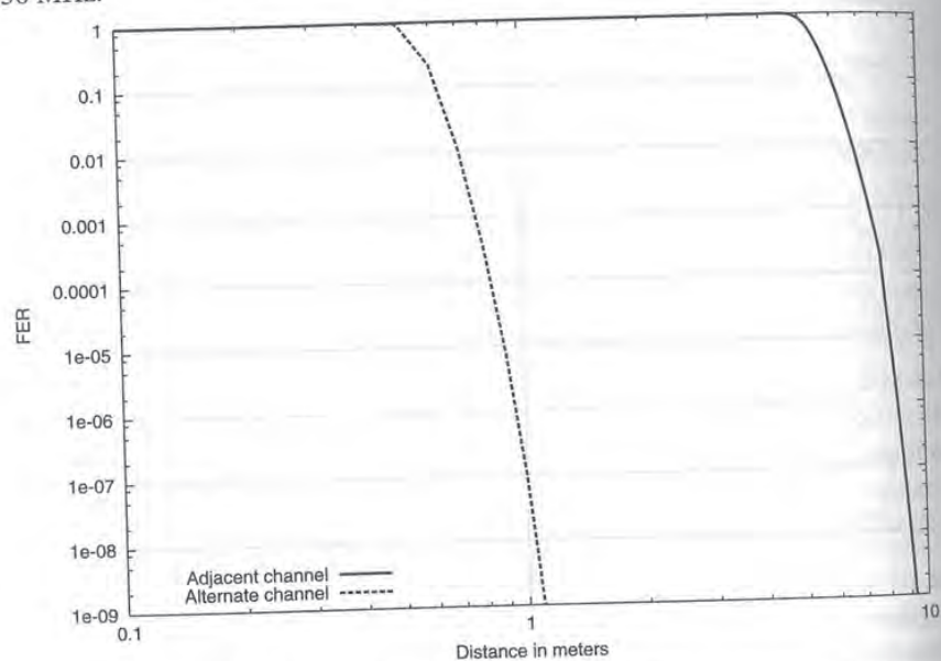
Figure 9-4: FER results for 802.15.3 with 802.11b as the interferer
