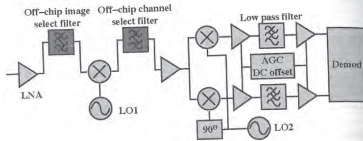
Figure 7-16: Superheterodyne radio architecture
