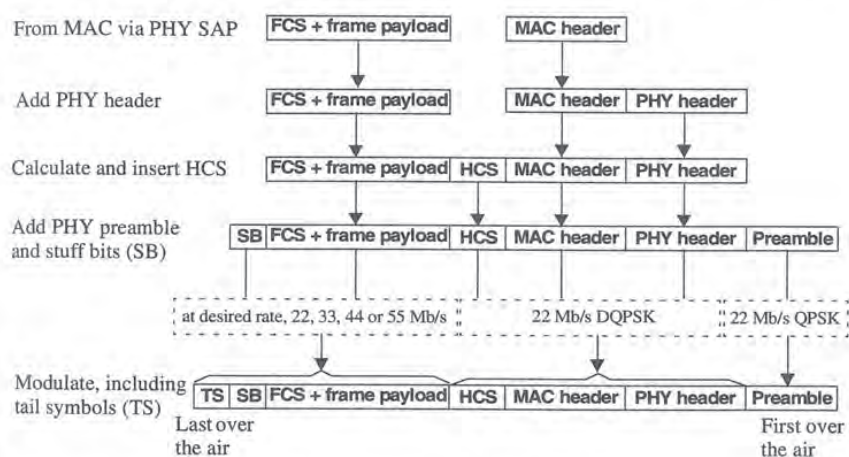
Figure 7-5: PHY frame formatting for 22-, 33-, 44-, and 55-Mb/s modes
