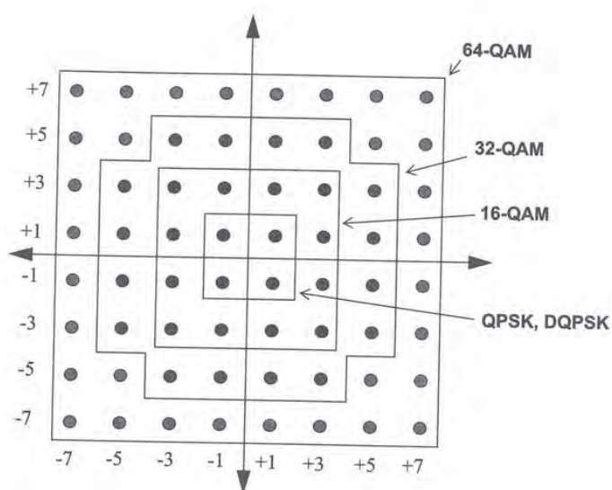
Figure 7-8: DQPSK, QPSK, 16/32/64-QAM signal constellations
