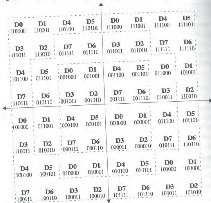
Figure 7-10: 16/32/64-QAM constellation bit mappings
