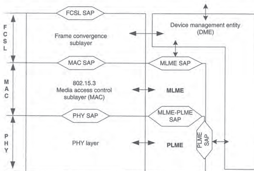
Figure 8-1: Reference model used in IEEE Std 802.15.3
