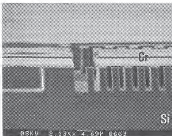
Figure 13: The BSM for suppressing RIE-lag.
