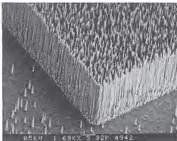
Figure 11: The forming of micrograss or black silicon.
