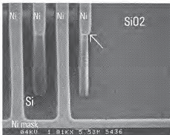
Figure 7: The influence of microloading.
