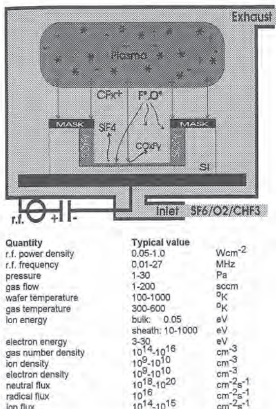
Figure 1: Basic RIE system and characteristics. 1 eV-8000 °K, 1 Pa-7.5 mTorr.
