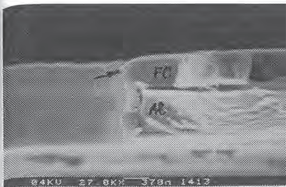
Figure 5: The effect of hydrogen addition; CHF 3 plasma (~CF 4 /H 2 ).
