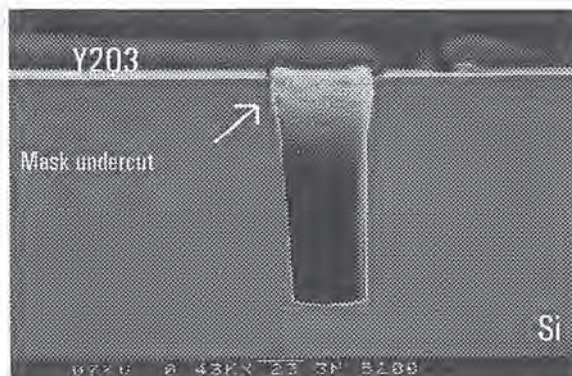
Figure 9: Undercutting of an \text{Y}_2\text{O}_3 mask due to ion bowing.
