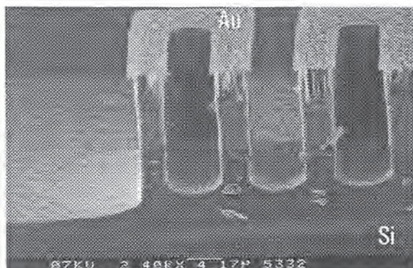
Figure 8: Mask erosion for a gold mask layer at 40eV.
