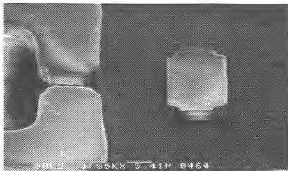
Figure 3: The two types of RIE etching. Left; ion-induced polymer etching. Right; ion-inhibitor Si etching with C_xH_y film at the beam-sidewalls.
