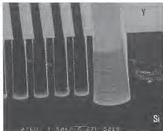
Figure 12: The influence of ion bowing on the profile.
