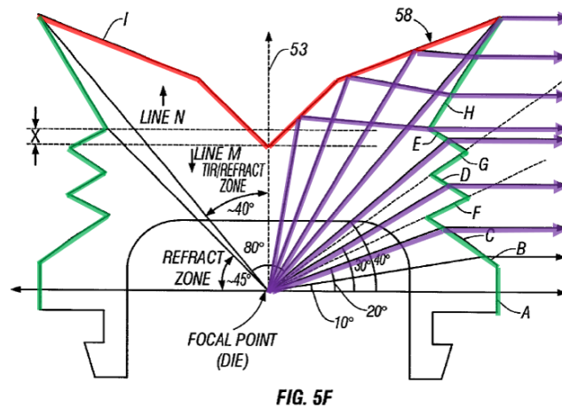
EX1005, Figure 5F. EX1002, ¶¶199-204.
