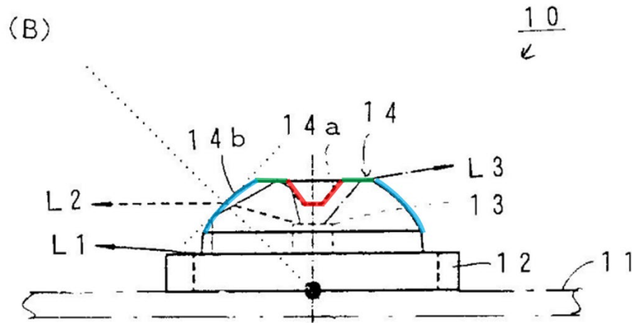
EX1004, Figure 1. EX1002, ¶¶52-55.
