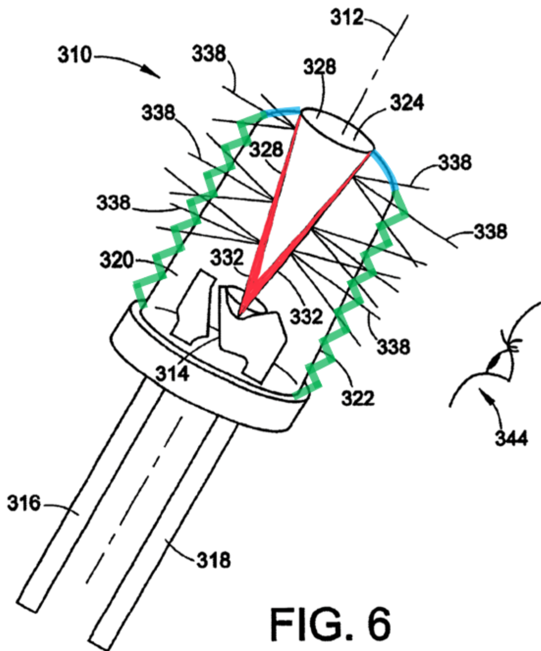
EX1006, Figure 6 (as modified with West). EX1002, ¶178.
