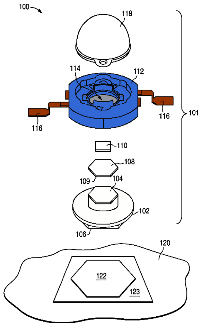
EX1007, Figure 1A. EX1002, ¶193.
