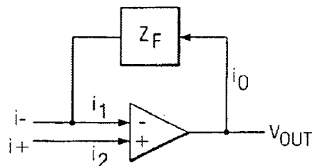
FIG. 7 (PRIOR ART)
