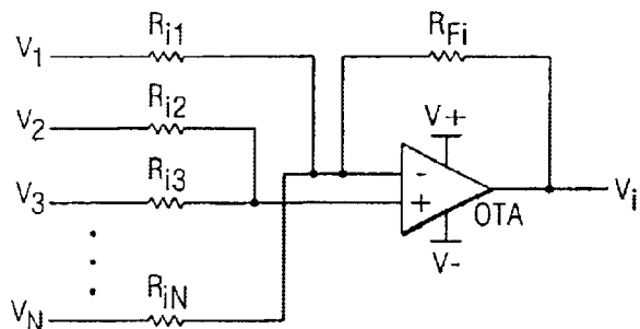
FIG. 7 (PRIOR ART)
