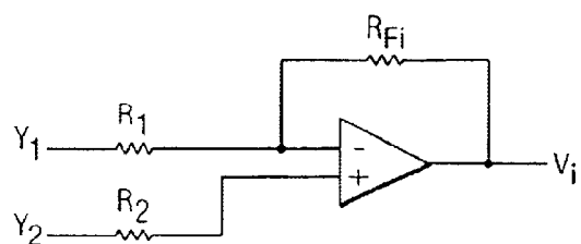
FIG. 8 (PRIOR ART)
