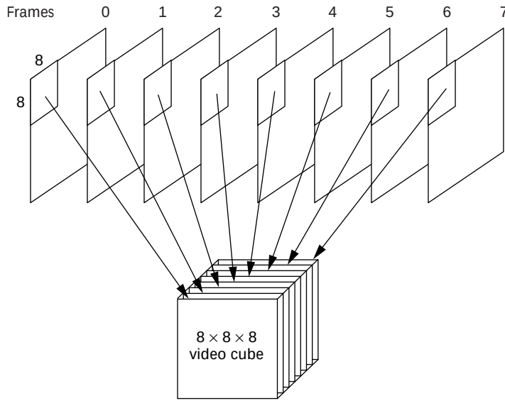
Figure 1. Forming an 8 \times 8 \times 8 video cube for XYZ compression.
