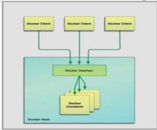
Figure 8. Docker architecture [58]
