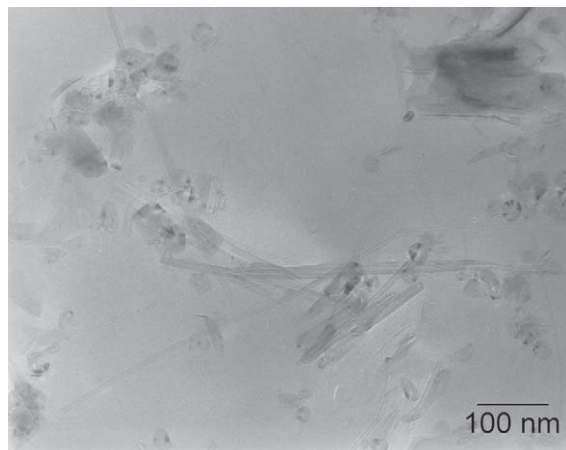
Fig. 1. TEM image of oxidised MWCNTs embedded in epoxy resin. The tubes are completely dispersed in the matrix due to the appearance of carboxylic groups on the surface.
