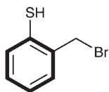
2-(bromomethyl)benzenethiol
