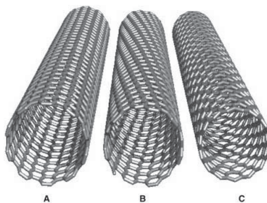
Figure 1. Idealized representation of defect-free (n,m) SWNTs with open ends. A) A metallic conducting (10,10) tube ("armchair"), B) a chiral, semiconducting (12,7) tube, and C) a conducting (15,0) tube ("zigzag"). The armchair (A) and zigzag (C) tubes are achiral. All the (n,m) armchair tubes are metallic, whilst this is only the case with chiral or zigzag tubes if (n-m)/3 is a whole number, otherwise, they are semiconductors. [1–4]
