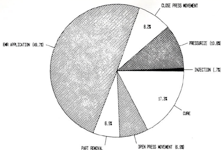
Figure 1. Typical RIM cycle measurements.
