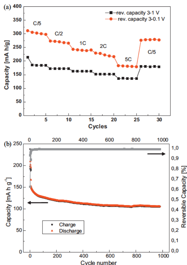
Fig. 4. Evolution of the reversible capacity from C/5 to 5 C in the potential window of 1–3 V (■) and 0.1–3 V (●) (a). Cycling stability and coulombic efficiency of 1000 cycles at a charging rate of 5 C (b) (first 5 cycles at C/5). (For interpretation of the references to color in this figure legend, the reader is referred to the web version of this article.)
