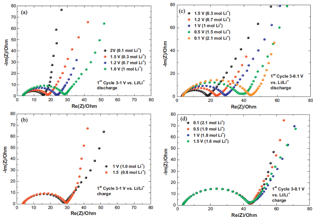
Fig. 7. Impedance spectra of the evaluated rutile samples: (a) 1st cycle discharge in the potential range of 3–1 V, (b) 1st cycle charge 3–1 V, (c) 1st cycle discharge 3–0.1 V, and (d) 1st cycle charge 0.1–3 V.
