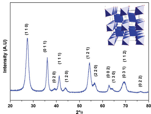
Fig. 2. XRD of the investigated \text{TiO}_2 sample after calcination. All reflexes can be assigned to rutile.
