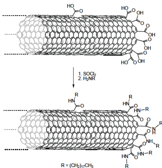
Scheme 1. Defect-group functionalization of SWNTs with octadecylamine. [14]
