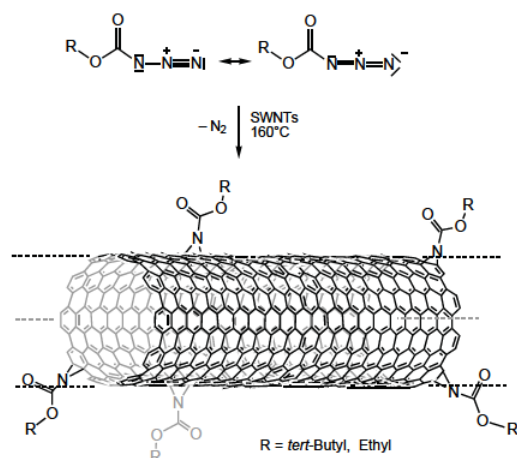
Scheme 2. Sidewall functionalization of SWNTs with alkyl azidoformates. [33]
