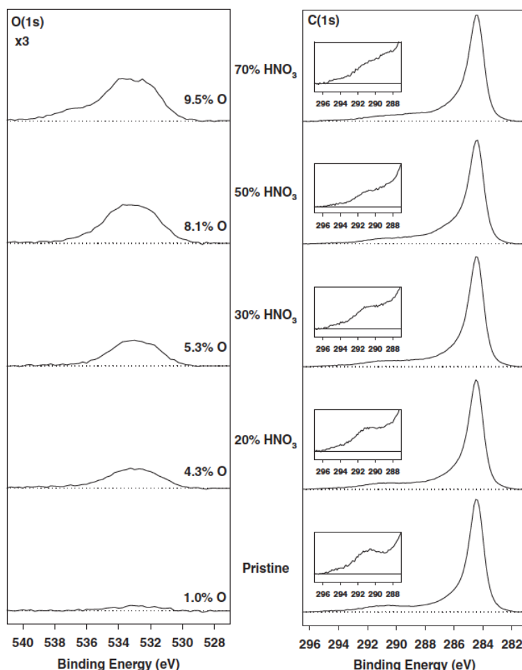
Fig. 6 – C(1s) and O(1s) XPS regions of MWCNTs oxidized by varying concentrations of \text{HNO}_3 . It should be noted that the O(1s) peaks have been normalized to the accompanying C(1s) peak areas in each case. The insert in the C(1s) region shows the \pi - \pi^* transition at \approx 291 eV.
