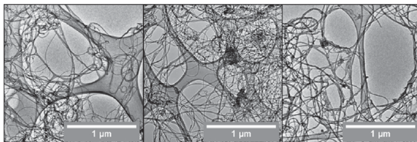
Fig. 4 – Low magnification TEM micrographs (left to right): pristine MWCNTs (0.9% O), O 3 treated MWCNTs (4.7% O), H 2 SO 4 /HNO 3 treated MWCNTs (10.2% O).
