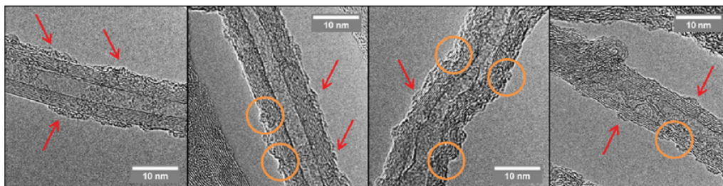
Fig. 10 – Representative TEM Micrographs (left to right): pristine MWCNTs (0.9% O), \text{H}_2\text{O}_2 treated MWCNTs (4.5% O), \text{H}_2\text{SO}_4/\text{HNO}_3 treated MWCNTs (5.1% O), \text{KMnO}_4 treated MWCNTs (5.3% O). Amorphous carbon is indicated with arrows, sidewall defects highlighted by circles.
