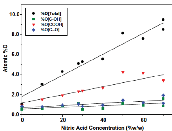
Fig. 7 – Influence of %w/w \text{HNO}_3 on the level of oxidation, as well as the distribution of oxygen-containing functional groups.
