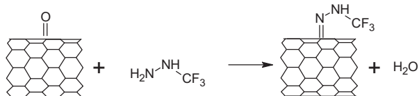
Fig. 3 – The selective reaction of carbonyl (C=O) groups with trifluoroethylhydrazine (TFH) to form a fluorinated hydrazone.
