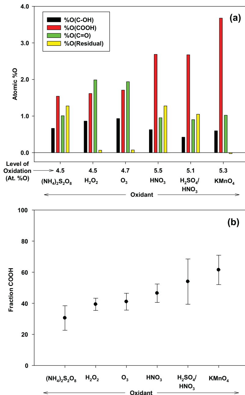
Fig. 9 – (a) Influence of the oxidant on the distribution of oxygen-containing functional groups, measured on MWCNTs that exhibit similar total oxygen concentrations. (b) Average and standard deviation for the percentage of COOH groups measured for each of the six oxidants, using different batches of MWCNTs treated under a range of different reaction conditions. For each oxidant at least three different batches of MWCNTs were treated; for \text{HNO}_3 and \text{H}_2\text{SO}_4/\text{HNO}_3 , 11 and 9 different batches were used, respectively.
