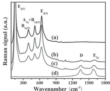
Fig. 4 Raman spectra of samples 1 (a), 3 (b), 5 (c) and MWCNTs (d).
