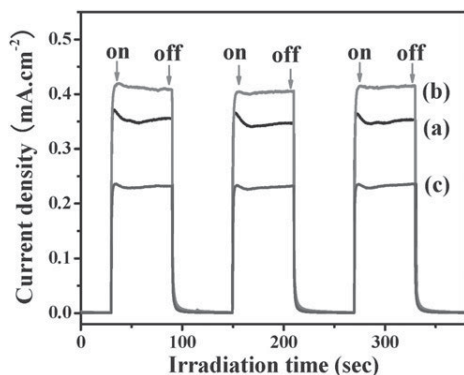
Fig. 11 The transient photocurrent responses of samples 1 (a), 3 (b) and 5 (c) in 1 M \text{Na}_2\text{SO}_4 aqueous solution under UV light irradiation at 0.5 V vs. Ag/AgCl.
