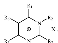
Pyrimidinium
