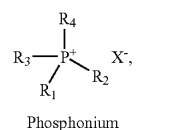
Phosphonium
