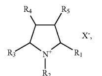
Pyrrolidinium
