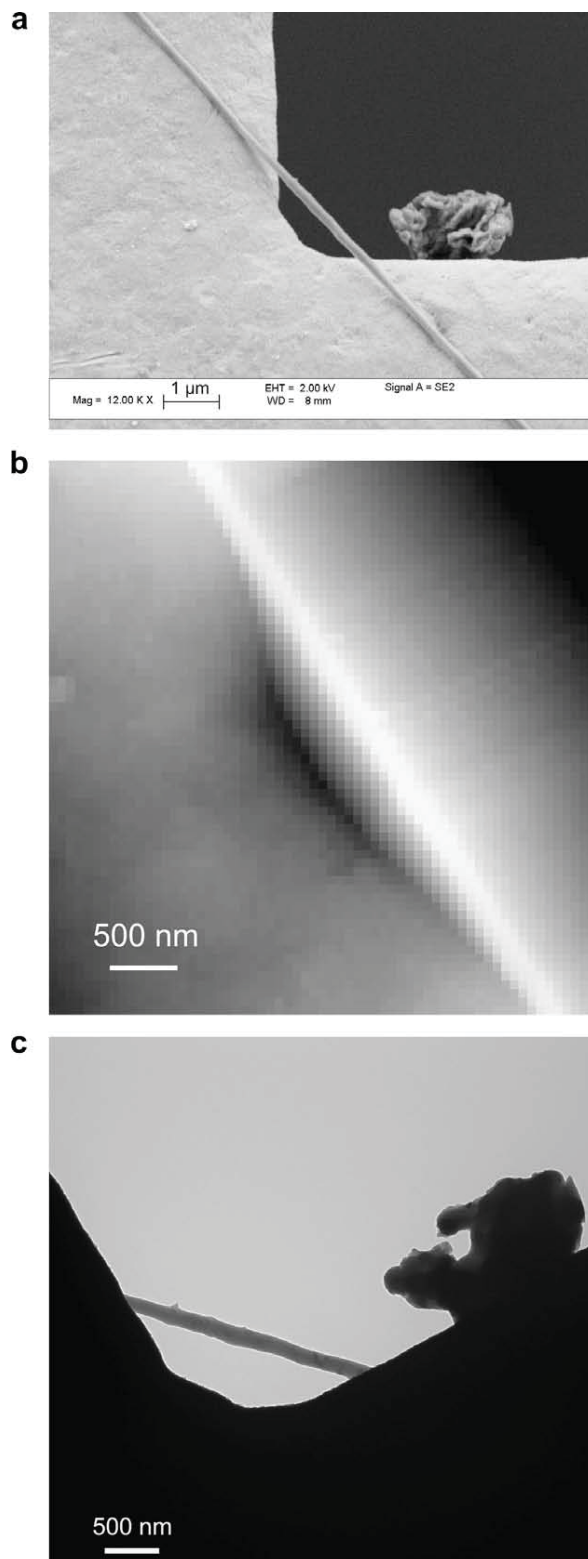
Fig. 2 – (a) SEM image, (b) AFM force-volume image, and (c) TEM image of the same PVA-LSA-CNT fiber suspended on a TEM grid.
