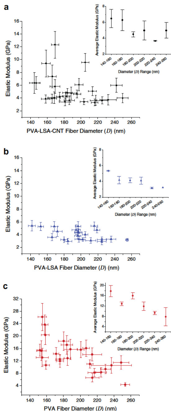
Fig. 3 – Plots of elastic modulus vs. diameter of: (a) 26 PVA-LSA-CNT, (b) 22 PVA-LSA and (c) 25 PVA fibers, with the inserts showing a profile of the average elastic modulus in each diameter range.
