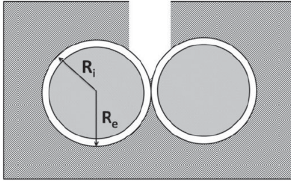
Fig. 8. Schematic representation of Haake batch mixer showing hydrodynamic radius ( R_i ) and external radius of the cavity ( R_e ).
