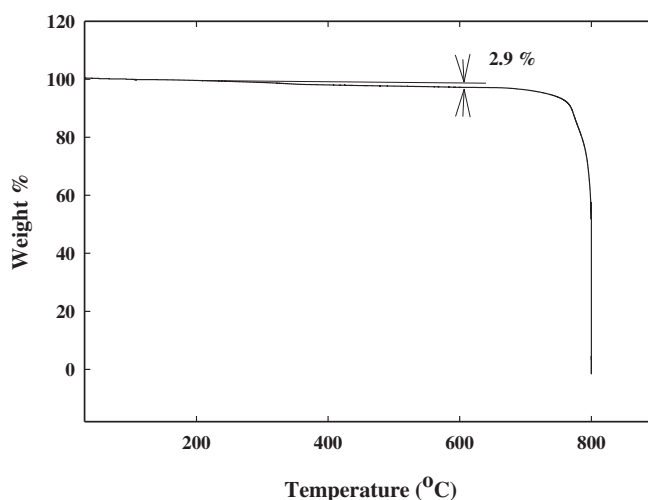
Fig. 2. Thermogravimetric analysis of oxidized MWCNTs.
