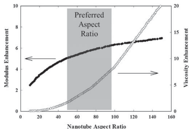
Fig. 1. Calculated modulus and viscosity enhancements of composites containing 10 wt.% MWCNT in a natural rubber matrix as a function of MWCNT aspect ratio.
