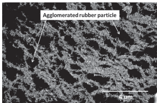
Fig. 6. SEM image of coagulated MWCNT-SBR masterbatch showing agglomerated SBR particles surrounded by MWCNTs.
