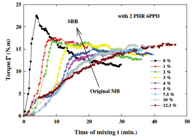
Fig. 11. Evolution of torque versus mixing time for 12.3 wt.% MWCNT-SBR masterbatch and various dilutions by adding SBR (Note: For convenience, the control SBR sample with no surfactant or MWCNT was prepared by the process described in the experimental section and is labeled as 0%).
