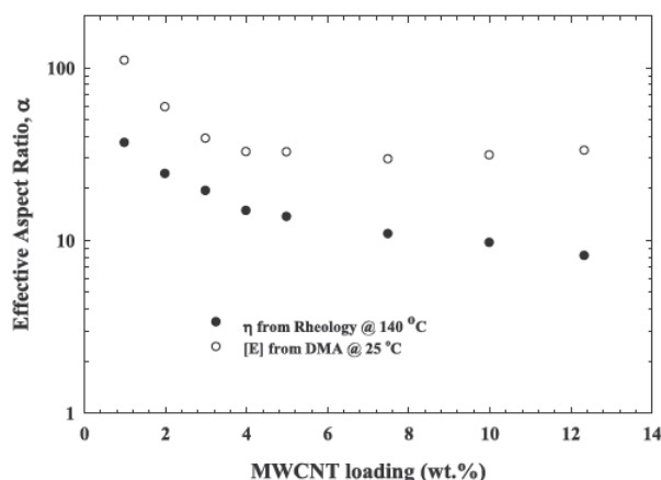
Fig. 20. Comparison of calculated aspect ratios calculated from rheology at 140 °C and DMTA at 25 °C.
