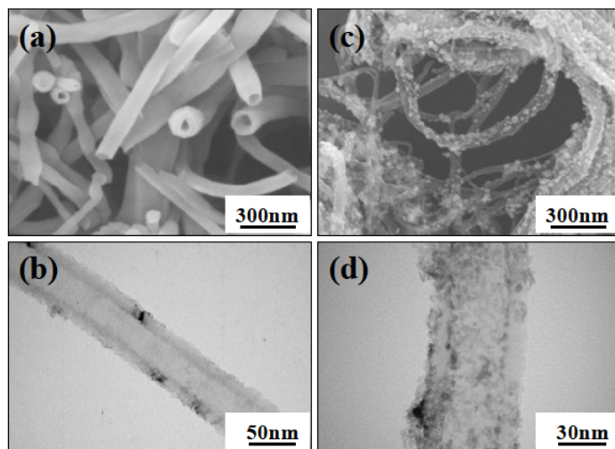
Figure 2. FE-SEM images of (a) original CNTs and (c) \text{SnO}_2/\text{CNT} composites. TEM images of (b) original CNTs and (d) \text{SnO}_2/\text{CNT} composites.
