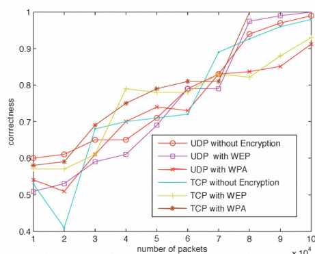
Figure 7. Fingerprinting for Defense - Cross-Traffic
