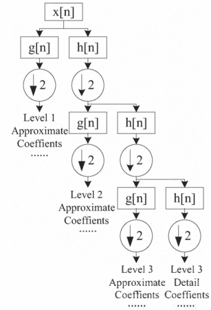
Figure 2. Wavelet filter
