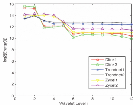
Figure 10. Energy graph of APs of three types)
