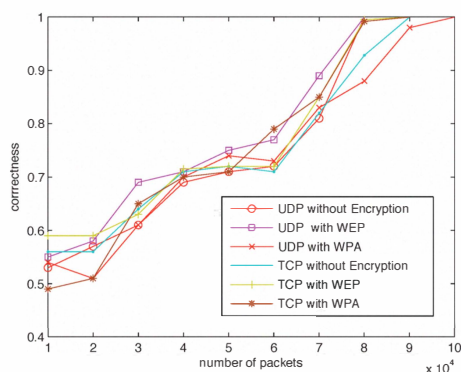
Figure 6. Fingerprinting for Defense - No Cross-Traffic
