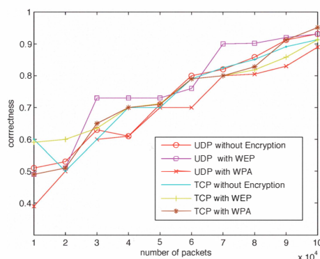
Figure 9. Offensive Fingerprinting - Cross-Traffic
