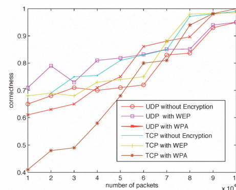
Figure 8. Offensive Fingerprinting - No Cross-Traffic
