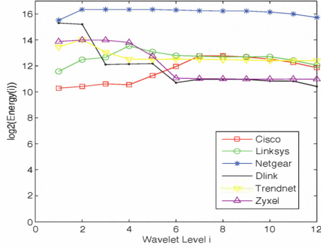
Figure 4. Energy graph of six APs
