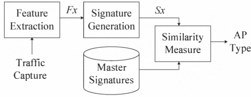
Figure 1. Overview of our approach
