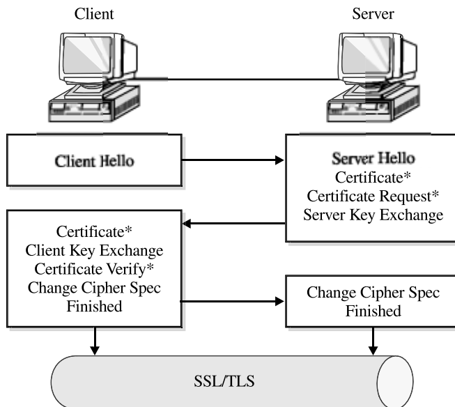
Figure 7-17 Overview of the handshake protocol
