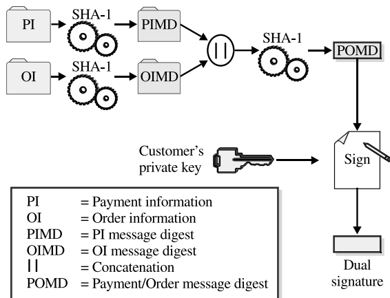
Figure 8-7 Generating dual signatures
