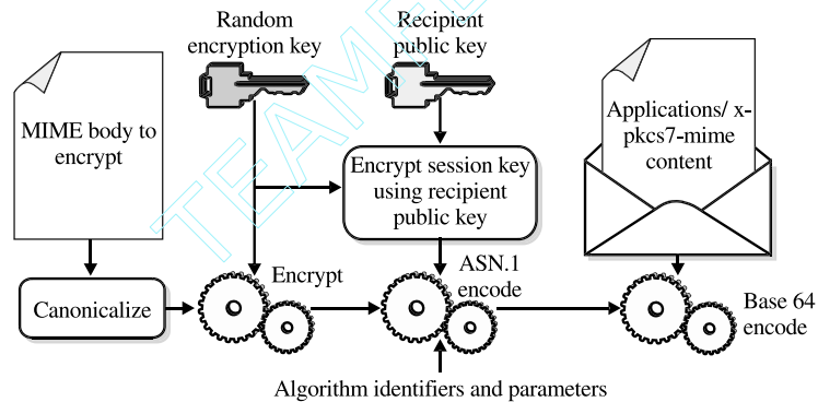
Figure 8-2 S/MIME enveloped-data process
