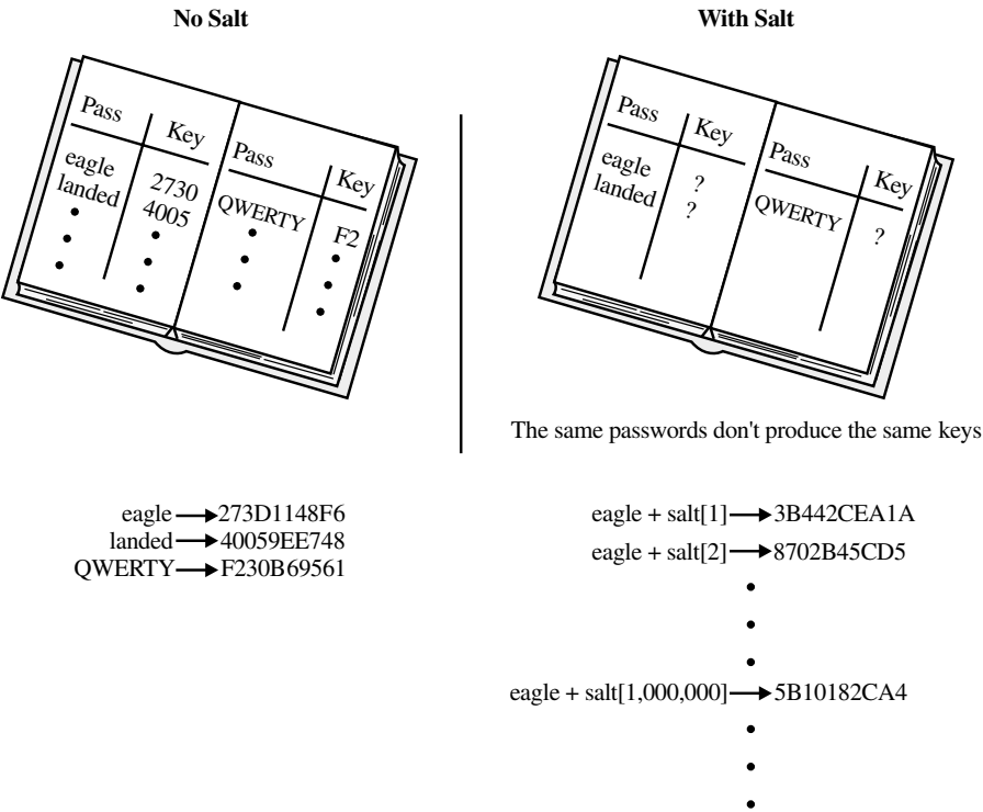
Figure 3-3 Using a salt foils a dictionary attack
