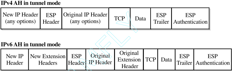
Figure 7-8 IPv4 and IPv6 header placement in tunnel mode
