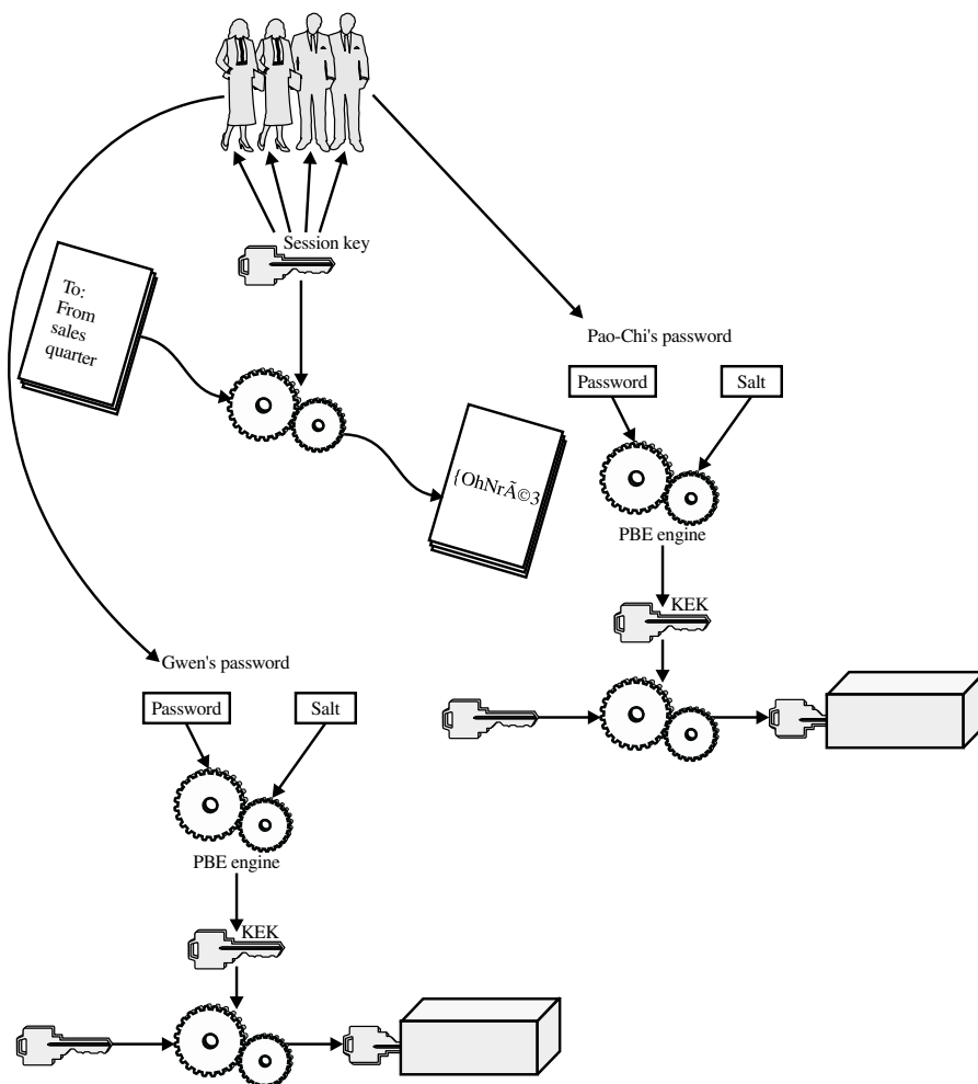
Using a session key for bulk data and protecting it with PBE means that users don't have to share passwords
