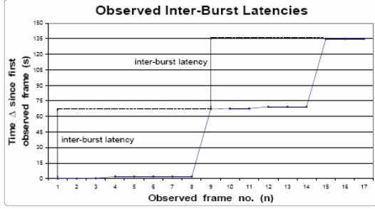
Figure 4: Inter-burst latency
