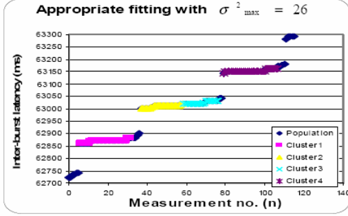
Figure 8: Appropriate Fitting with suitable \sigma^2_{\max}
