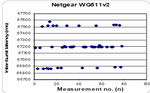
Figure 6: Inter-burst latencies of Netgear WG511v2
