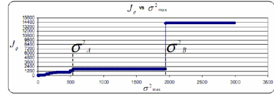
Figure 7: J_e as a function of \sigma_{\max}^2
