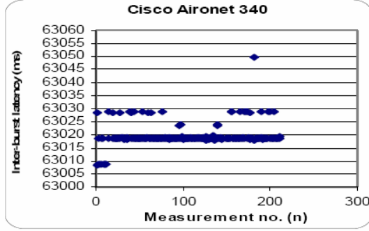
Figure 5: Inter-burst latencies of Cisco Aironet 340
