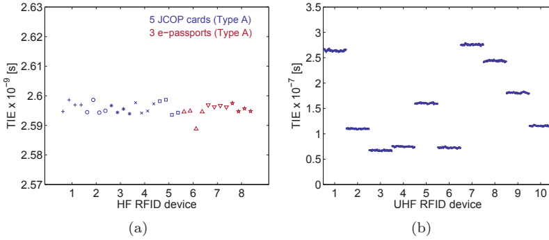
Figure 5.9: Timing feature for HF and UHF RFID. (a) HF RFID smart cards and e-passports of the same type exhibit stable, but indistinguishable time interval errors (TIE). (b) Same type UHF RFID tags present stable and distinguishable TIE over different configurations.
