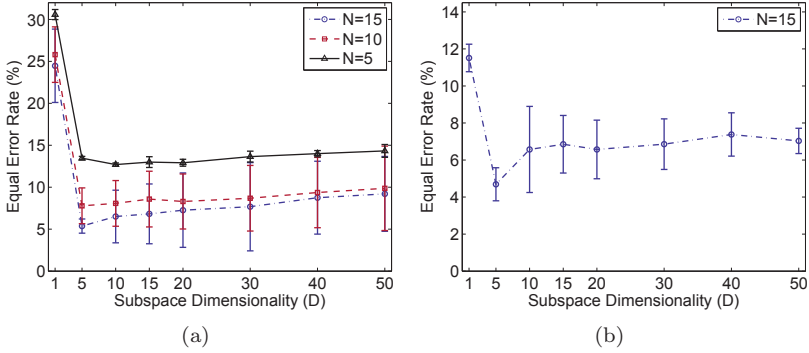
Figure 5.6: Spectral features identification accuracy for N identification signals used to build the fingerprint and feature dimensionality D (Dataset 2). (a) Burst spectral features (b) Sweep spectral features
