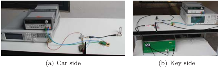
Figure 2.5: Experimental relay over-the-air realization.
