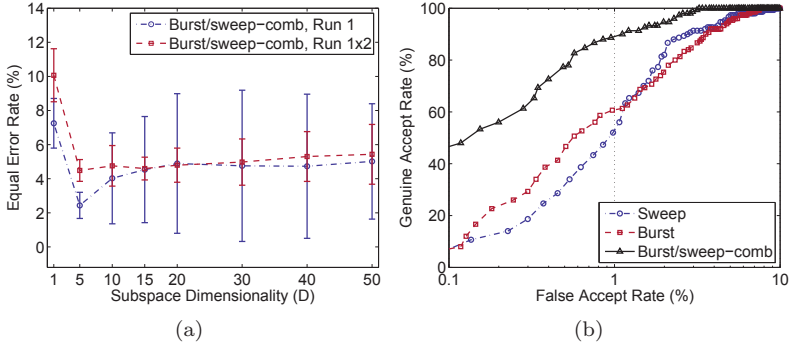
Figure 5.8: (a) Identification accuracy by combining the sweep and burst features (b) Receiver operating characteristic (ROC) for burst and sweep spectral features and their combination (Dataset 2, D = 5 and N = 15 ). See Table 5.5 for the underlying data.
