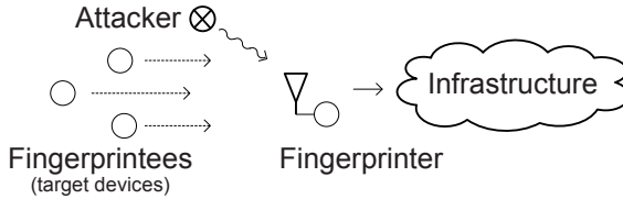
Figure 7.1: Our system consists of a wireless network with a number of wireless devices (fingerprints) and a fingerprinting device (fingerprinter). We assume that in the system initialization phase the fingerprints of the devices are registered with the fingerprinter. The fingerprints are extracted from the packets sent by the devices and verified by the fingerprinter. The goal of the attacker is to impersonate a target device by generating packets that contain the fingerprints of that device.
