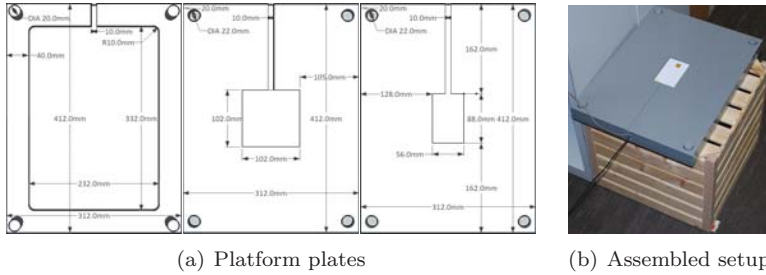
Figure 6.2: Antenna setup. The setup consists of a platform with three plates that hold two antennas and the device to be measured. The bottom plate holds a pad-style transmission antenna, the middle plate holds the acquisition antenna and the top plate provides a slot for placing devices (smart cards).
