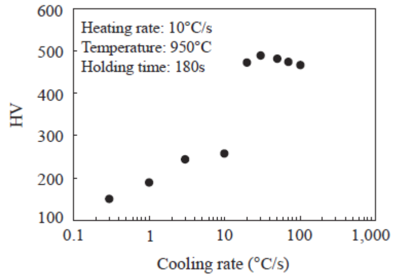
Fig. 4 Influence of cooling rate on hardness
