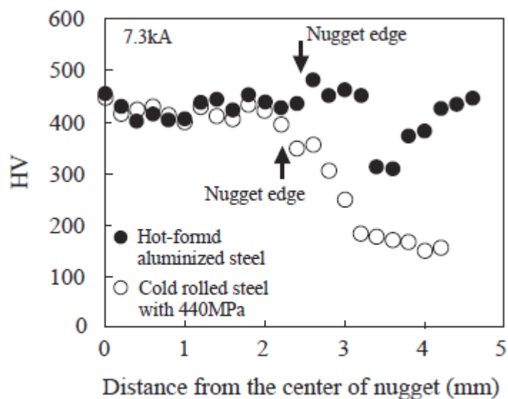
Fig. 10 Hardness distribution near spot-welded portion
