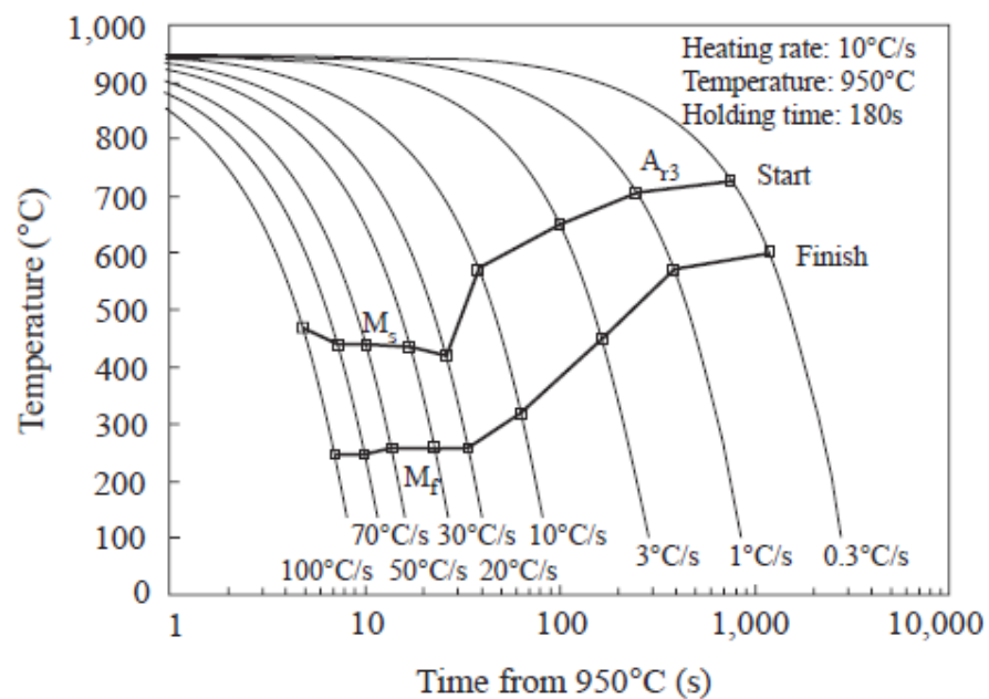
Fig. 3 CCT curves
