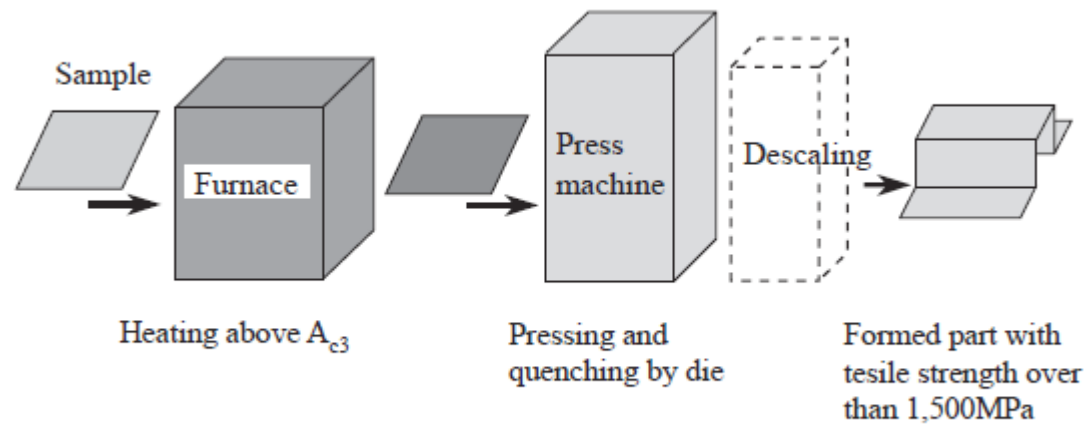
Fig. 1 Schematic illustration of hot forming process
