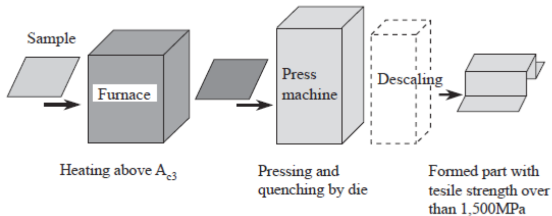
Fig. 1 Schematic illustration of hot forming process
